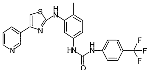
012: 1-(4-Fluoro-phenyl)-3-[4-methyl-3-(4-pyridin-3-yl-thiazol-2-ylamino)-phenyl]-urea
