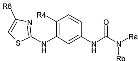
FORMULA II-2
