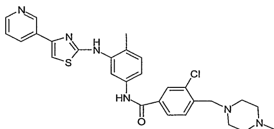
079: 3-Chloro-4-(4-methyl-piperazin-1-ylmethyl)-N-[4-methyl-3-(4-pyridin-3-yl-thiazol-2-ylamino)-phenyl]-benzamide
