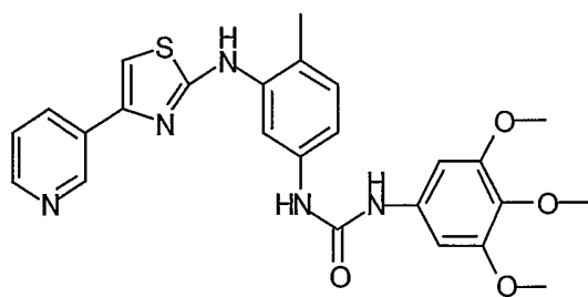
013: 1-[4-Methyl-3-(4-pyridin-3-yl-thiazol-2-ylamino)-phenyl]-3-(3,4,5-trimethoxy-phenyl)-urea
