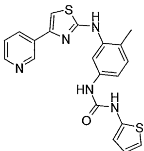
015: 1-[4-Methyl-3-(4-pyridin-3-yl-thiazol-2-ylamino)-phenyl]-3-thiophen-2-yl-urea
