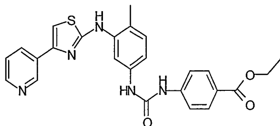
015: 1-[4-Methyl-3-(4-pyridin-3-yl-thiazol-2-ylamino)-phenyl]-3-thiophen-2-yl-urea
