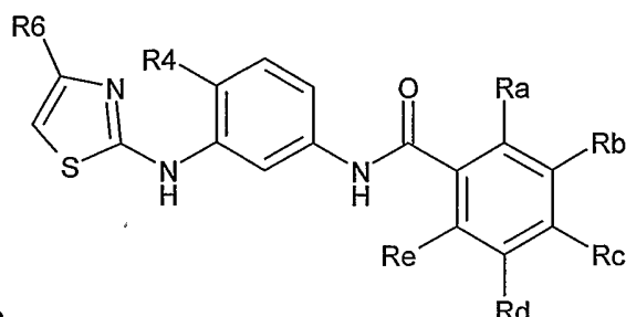
FORMULA II-3
