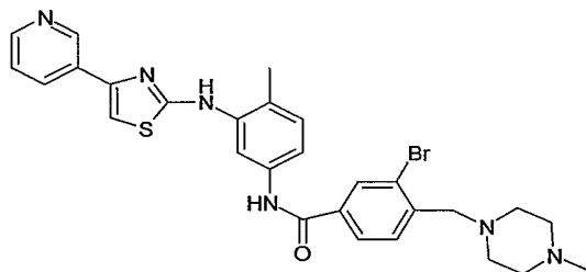
078: 3-Bromo-4-(4-methyl-piperazin-1-ylmethyl)-N-[4-methyl-3-(4-pyridin-3-yl-thiazol-2-ylamino)-phenyl]-benzamide
