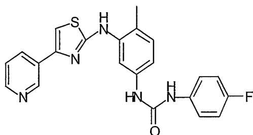
012: 1-(4-Fluoro-phenyl)-3-[4-methyl-3-(4-pyridin-3-yl-thiazol-2-ylamino)-phenyl]-urea
