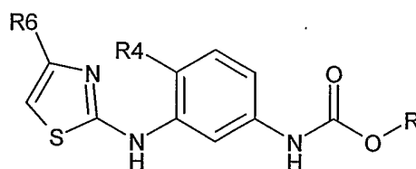
FORMULA II-6
