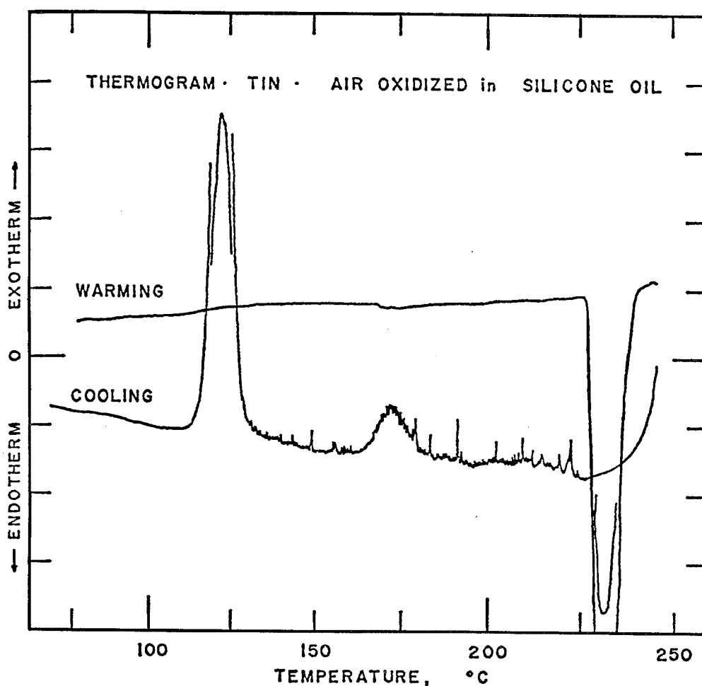
FIG. 3 Thermogram for pure tin. Emulsion formed by air oxidation in silicone oil. Melting point, 232°C. Thermogram peak crystallization temperature, 124°C. Peak supercooling, 108 degrees. Supercooling range, 20 degrees.
