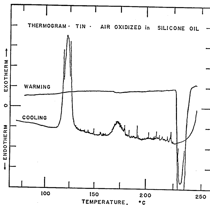
Thermogram for pure tin. Emulsion formed by air oxidation in silicone oil. Melting point, 232°C. Thermogram peak crystallization temperature, 124°C. Peak supercooling, 108 degrees. Supercooling range, 20 degrees.
