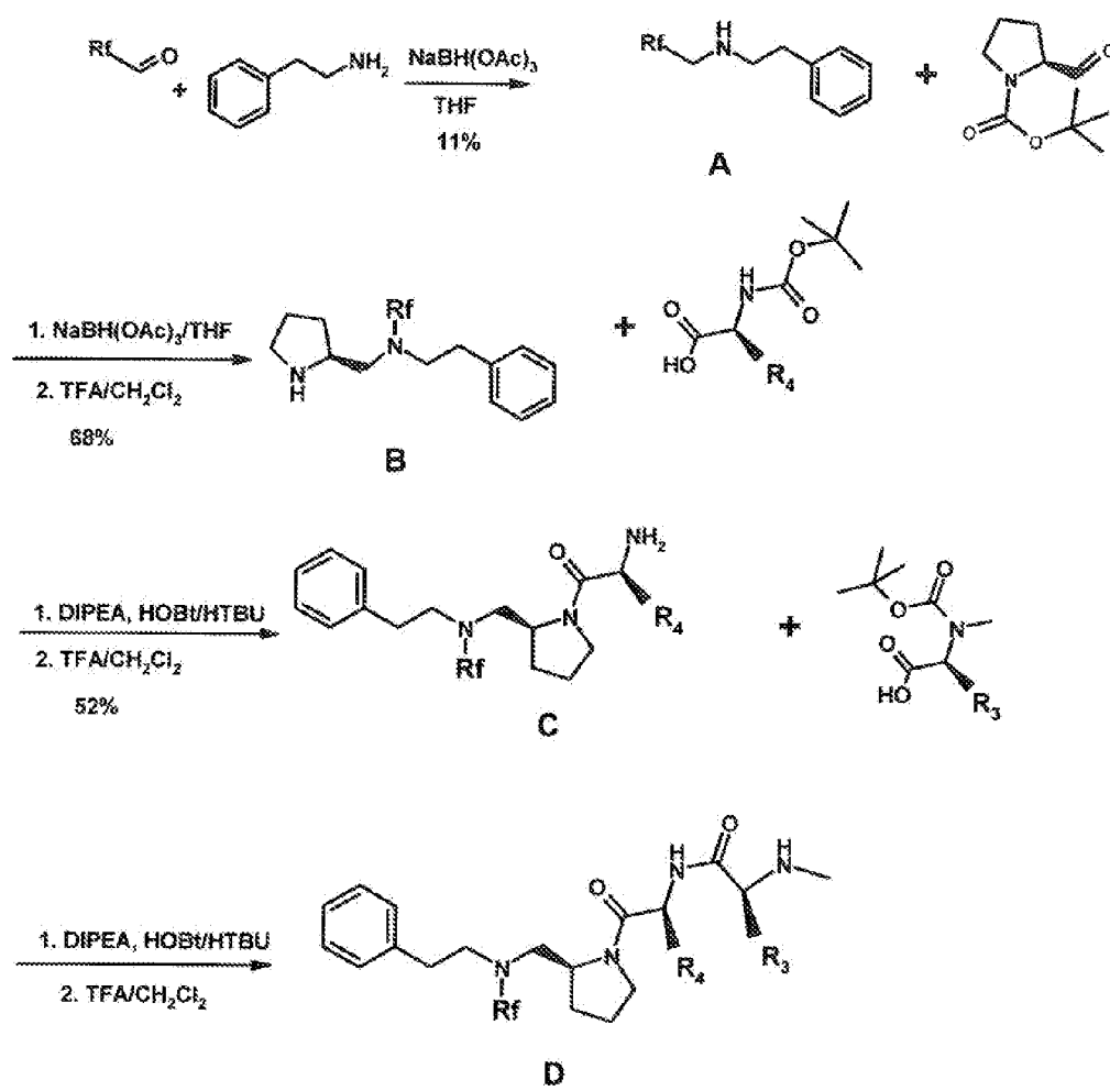
Scheme 2
