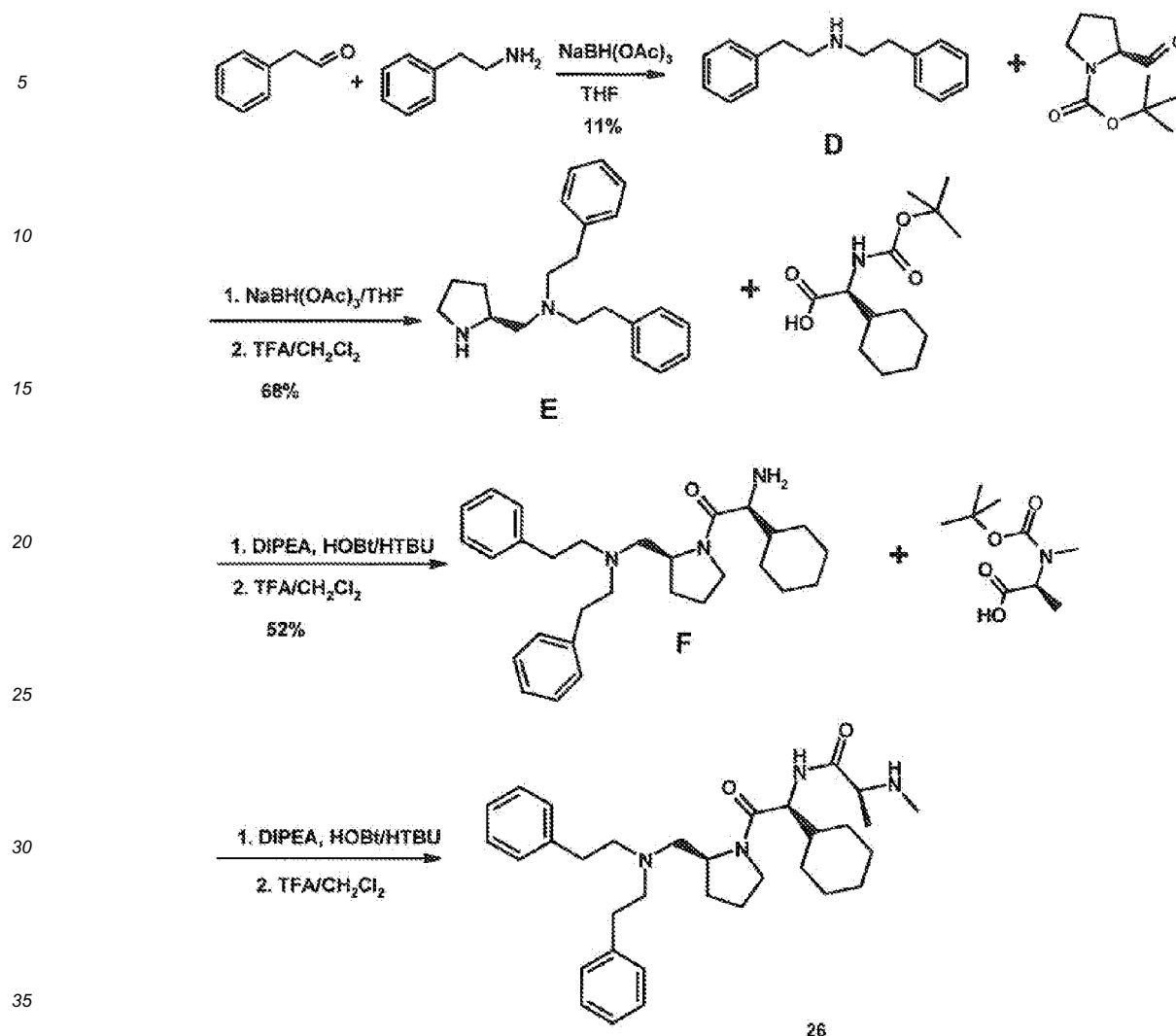
Scheme 6
