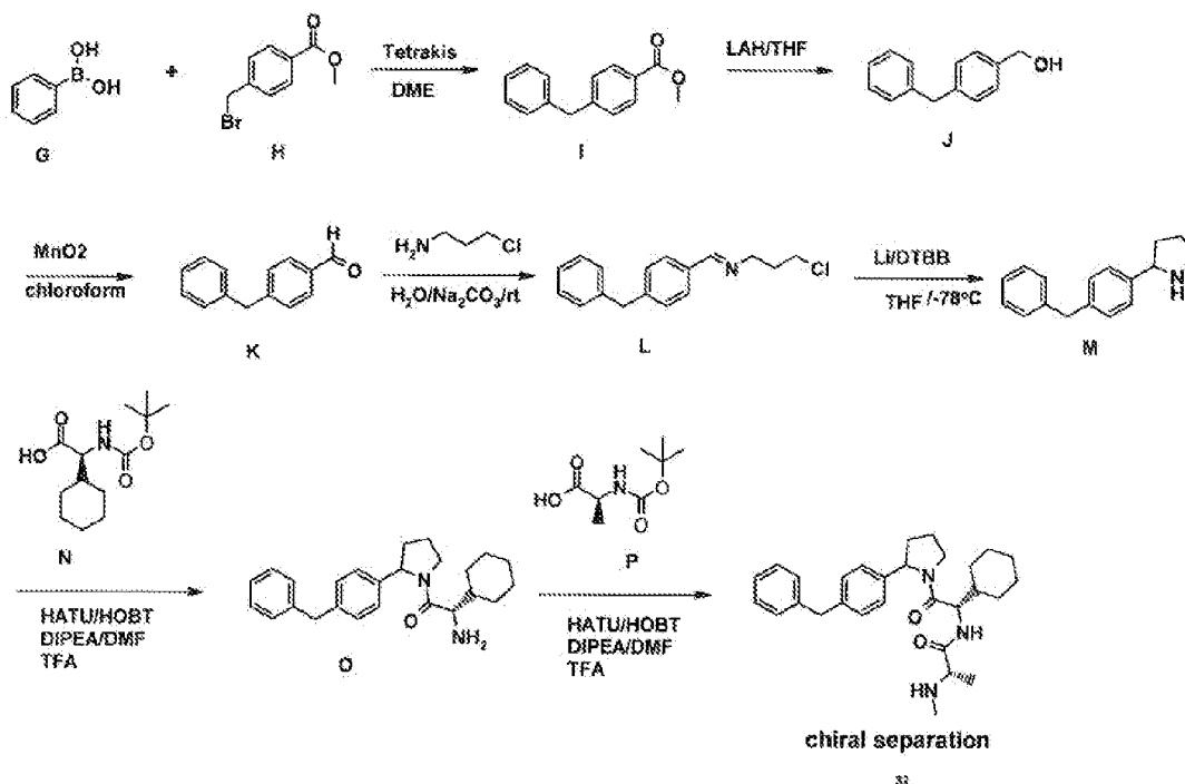
Scheme 7
