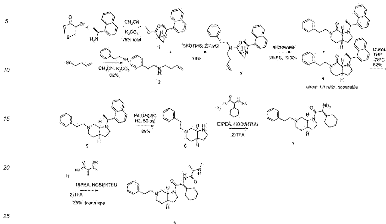
Scheme 5
