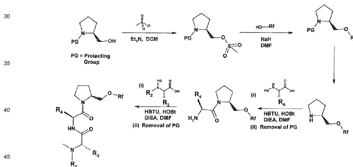
Scheme 4
