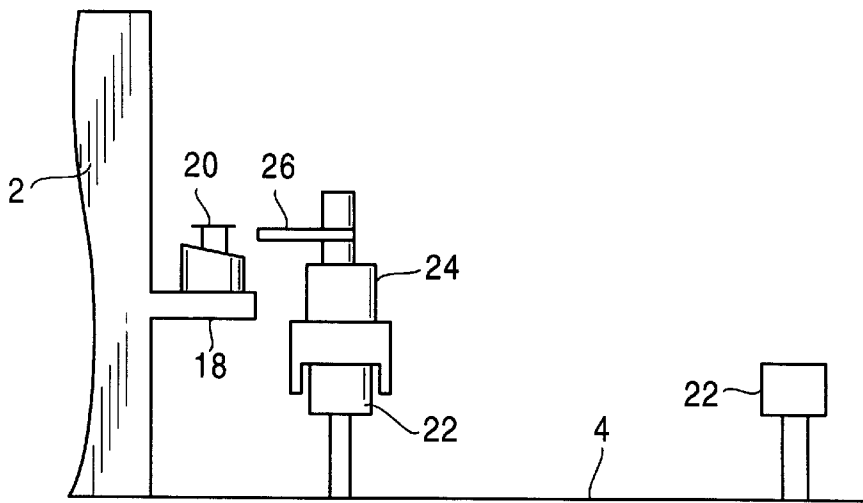
FIG. 7 PRIOR ART
