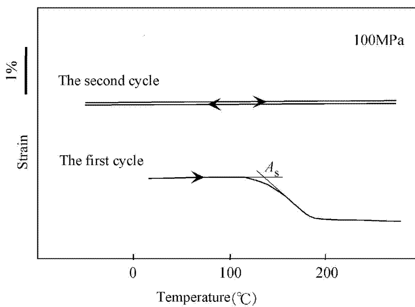
Fig. 1B The typical strain versus temperature curve of the comparative alloys
