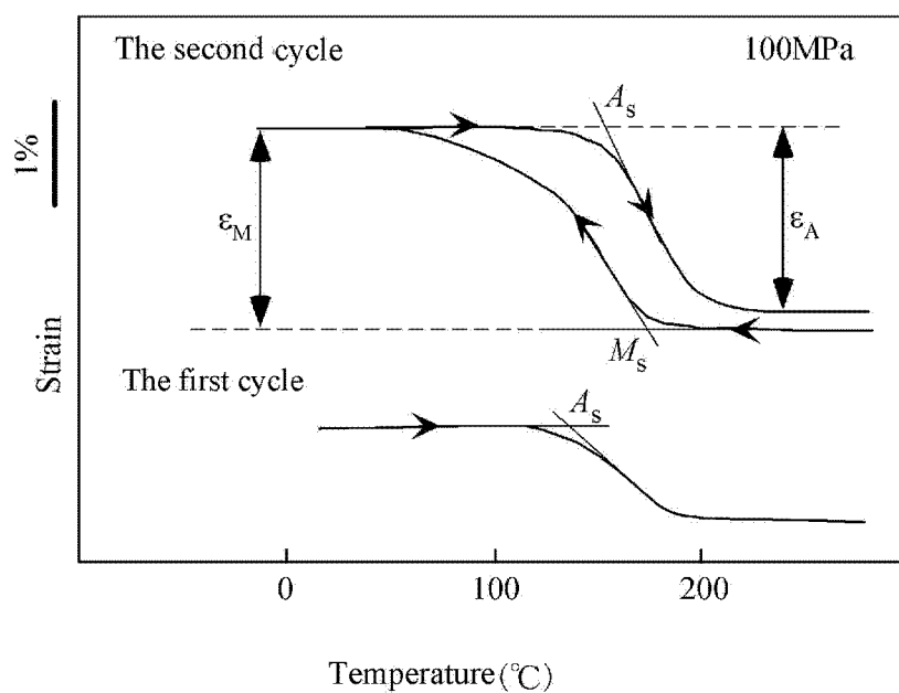
Fig. 1A The typical strain versus temperature curve of the invented alloys
