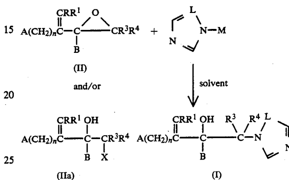
Scheme I
