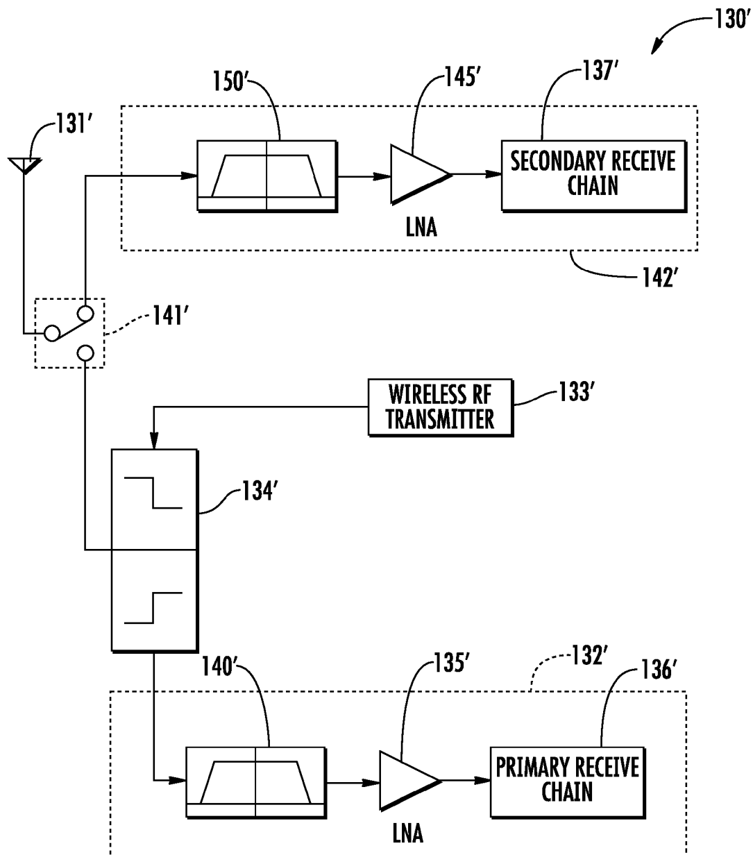
FIG. 6 (PRIOR ART)
