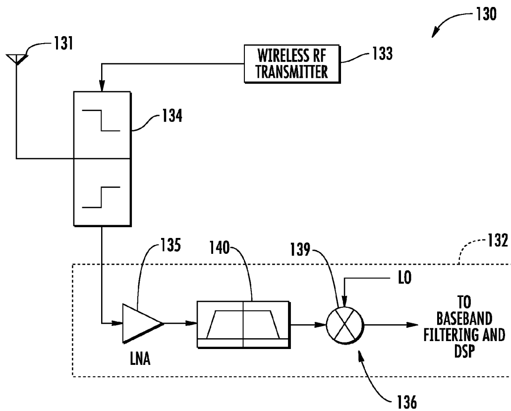
FIG. 5 (PRIOR ART)
