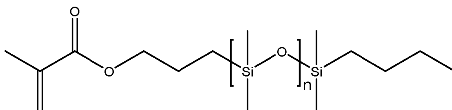
Formula III (mPDMS)
