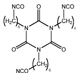
HDI isocyanurate (HDI trimer)
