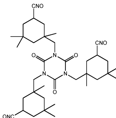
IPDI isocyanurate (IPDI trimer)
