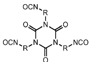
isocyanurate trimer
