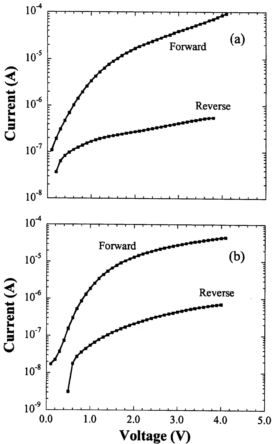
Figure 20(a) and 20(b): I/V characteristic in the dark of the sample formed (a) at 355 nm and (b) at 532 nm.
