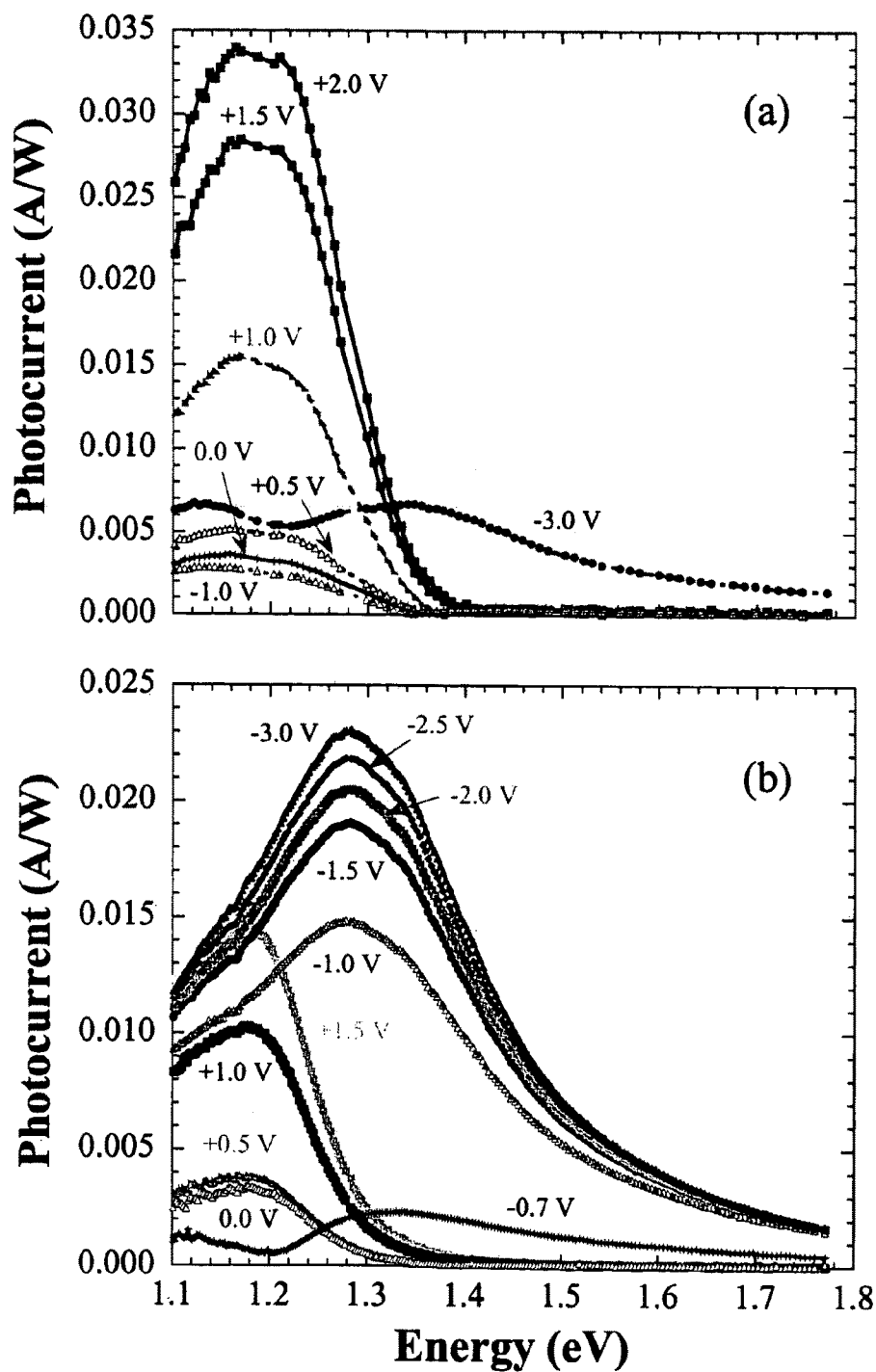
Figures 18(a) and 18(b): (a) PC of the sample formed at 355 nm and (b) PC of the sample formed at 532 nm for various forward (+) and reverse biases.
