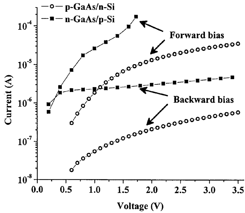
Figure 13: I/V characteristic of the p-GaAs/n-Si and n-GaAs/p-Si sample.
