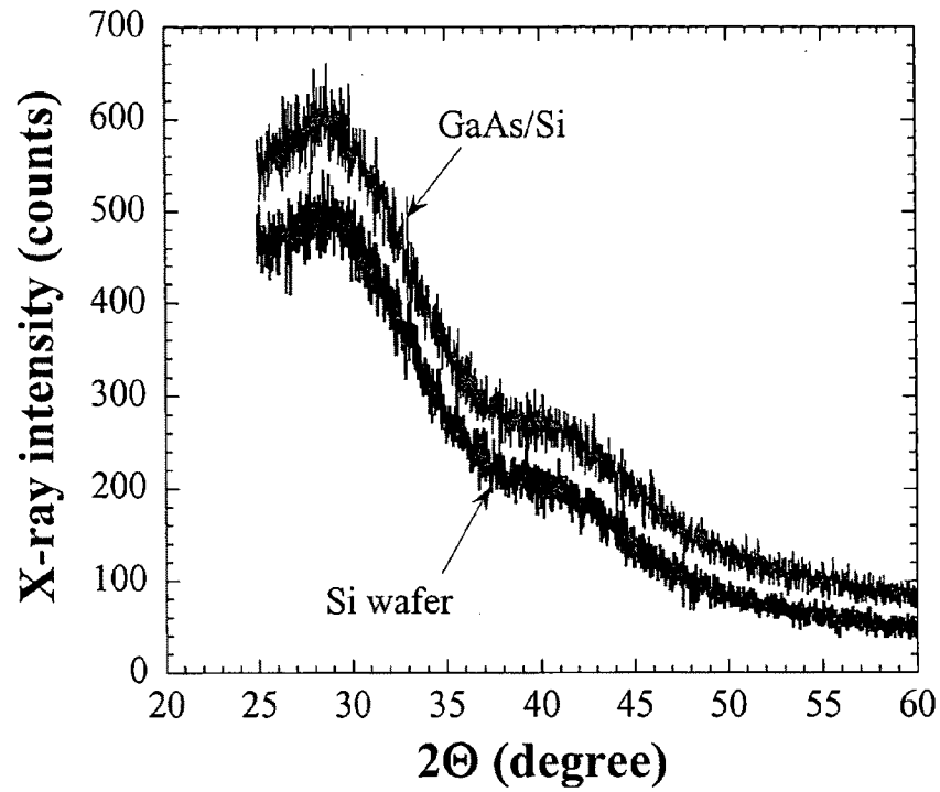
Figure 23: X-ray signal of the film formed at 1064 nm and of a Si substrate without film.
