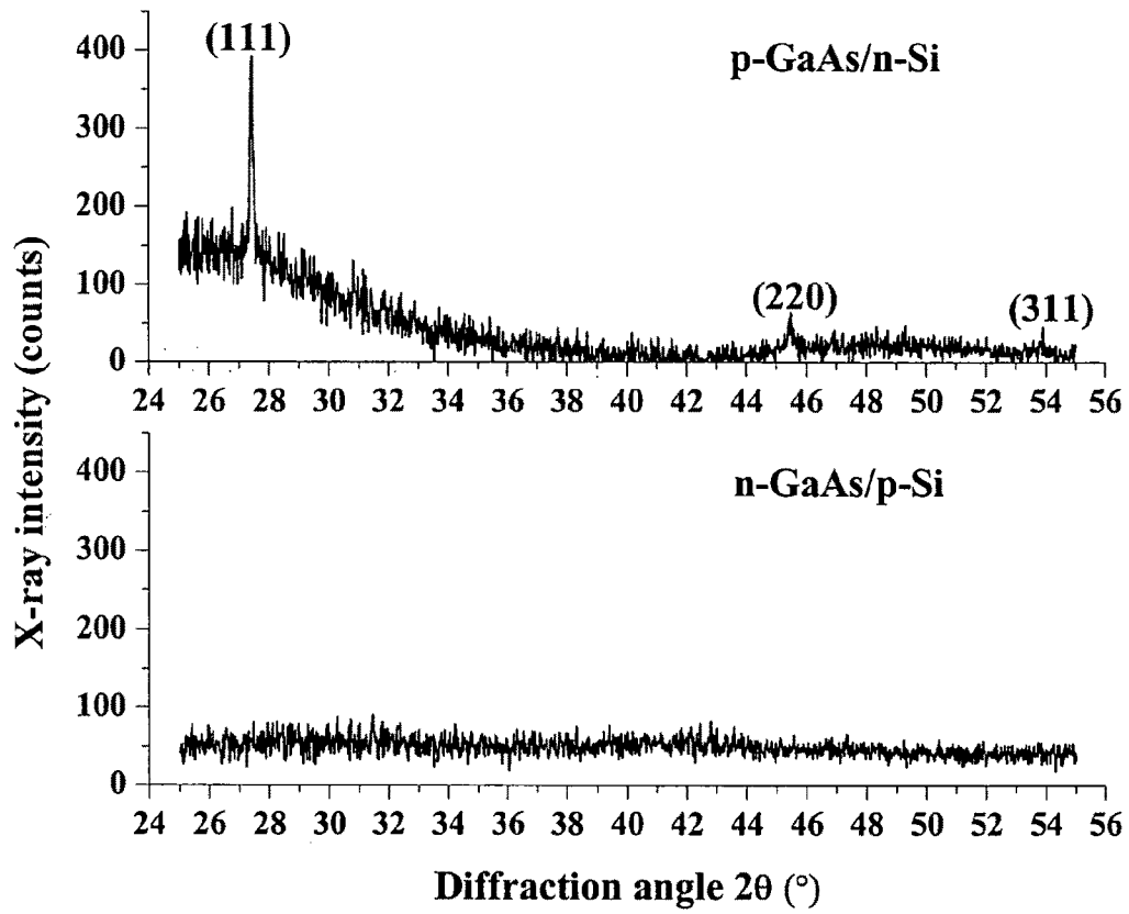
Figure 10: X-ray diffraction patterns for both samples. The background signal of the substrate has been subtracted.
