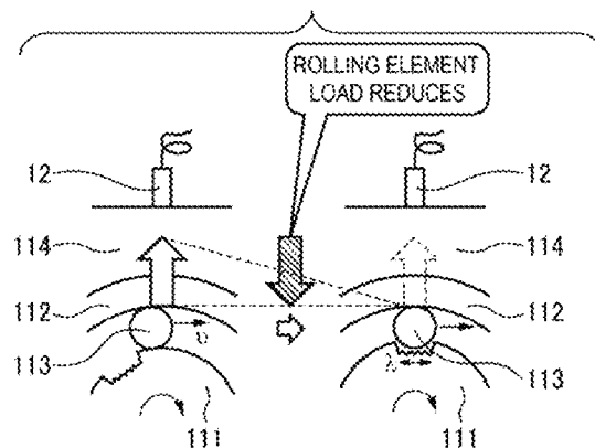
WHEN ROLLING ELEMENT ENTERS FLAKING
