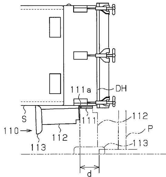
Fig.9 (Prior Art)
