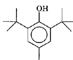
(R-28)
