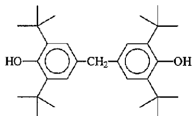
(R-32)
