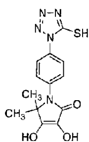
(39)
