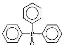
(D-1)
