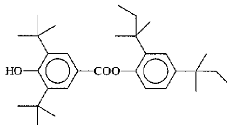
(R-30)
