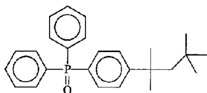
(D-19)
