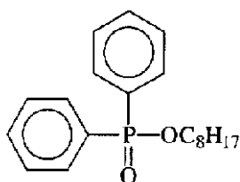
(D-17)
