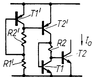
Fig. 3. PRIOR ART
