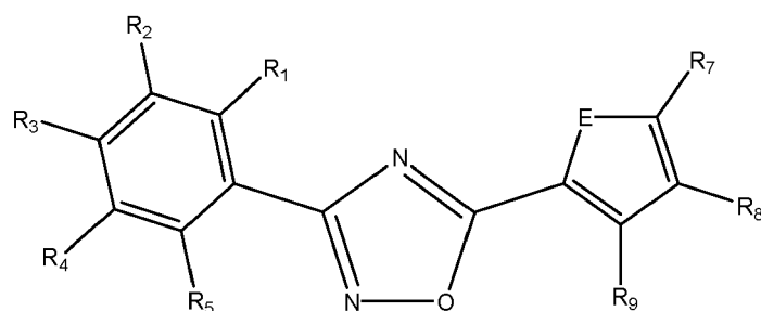
Formula IVa
