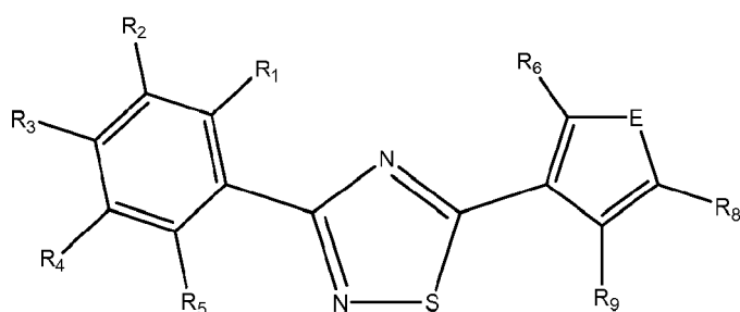
Formula VIb
