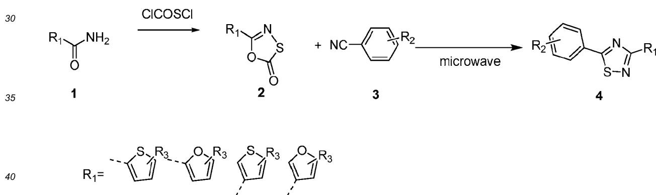
Scheme 7: Synthetic scheme to compounds of the Formula VIIa and VIIb
