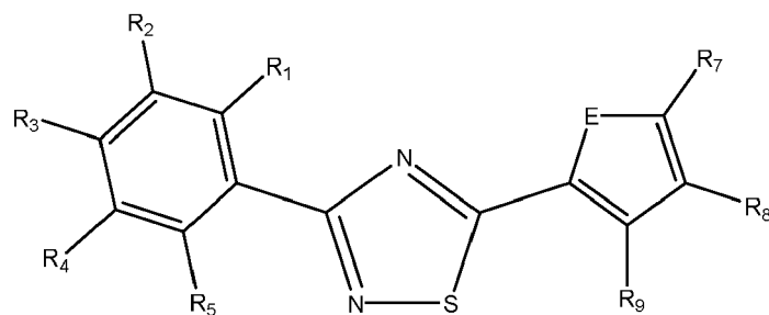
Formula VIa
