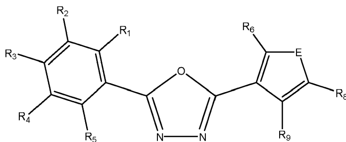
Formula IIIb
