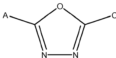
Formula III
