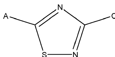
Formula VII
