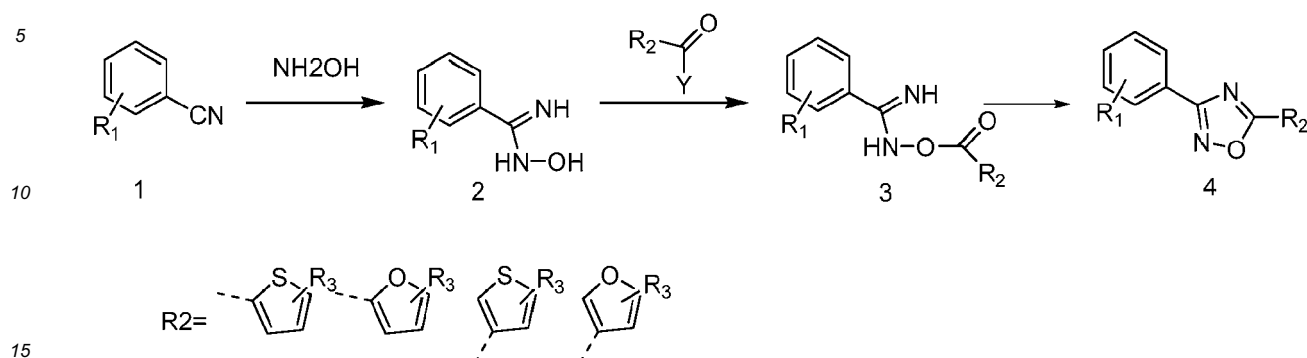
Scheme 4: Synthetic scheme to compounds of the Formula IVa and IVb
