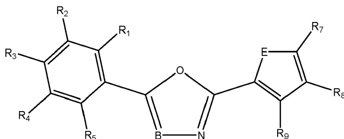
Formula Ia
