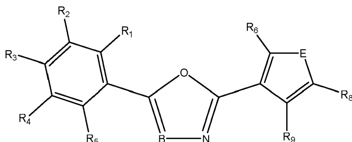
Formula Ib
