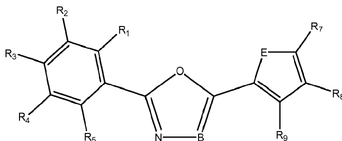
Formula IIa
