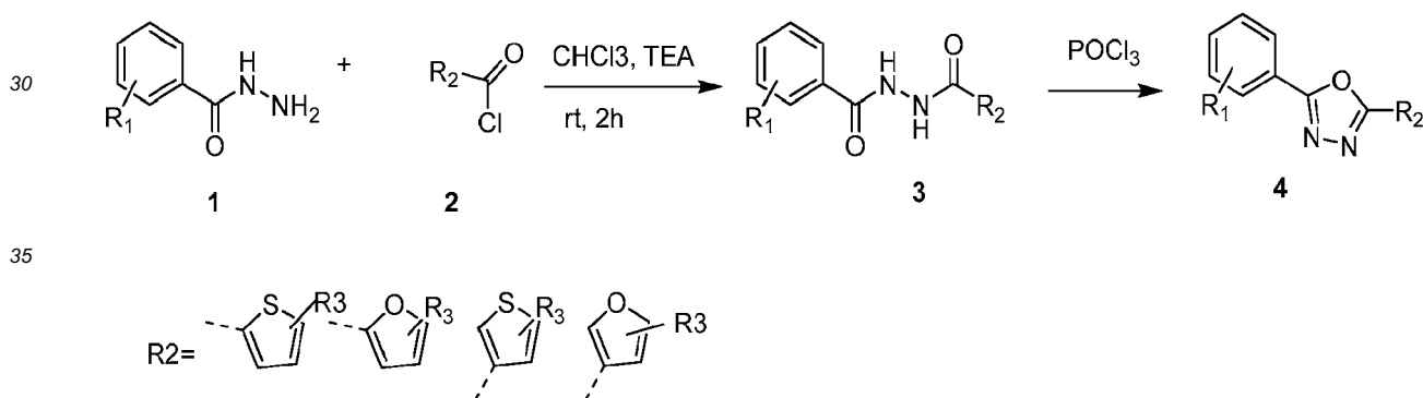
Scheme 3: Synthetic scheme to compounds of the Formula IIIa and IIIb
