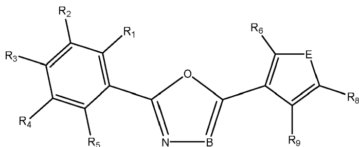
Formula IIb
