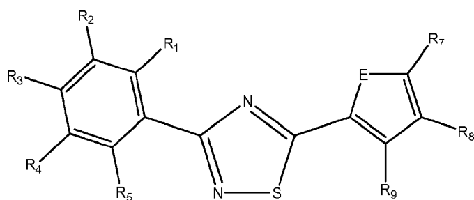
Formula VIa
