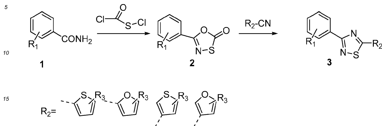
Scheme 6: Synthetic scheme to compounds of the Formula VIa and VIb
