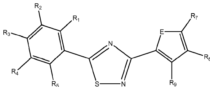
Formula VIIa
