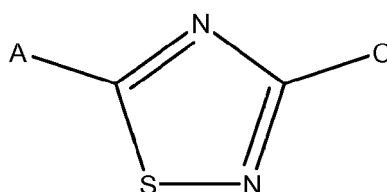
Formula VII
