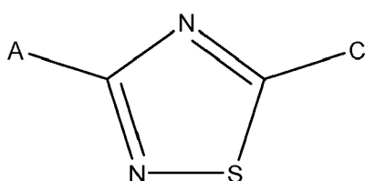
Formula VI
