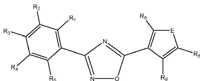
Formula IVb
