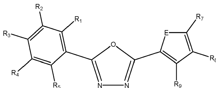
Formula IIIa
