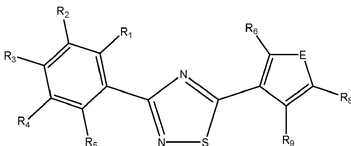
Formula VIb
