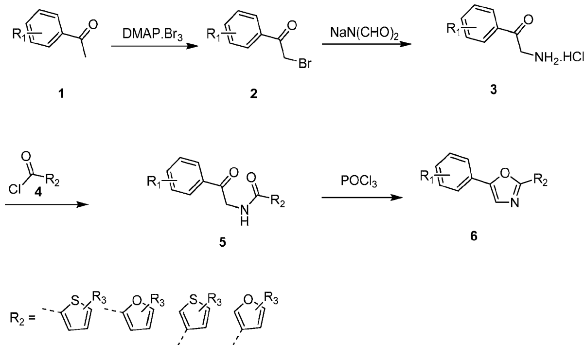
Scheme1: Synthetic scheme to compounds of the Formula Ia and Ib
