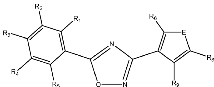
Formula Vb
