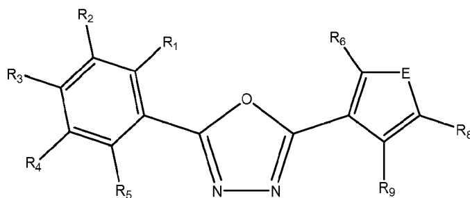
Formula IIIb
