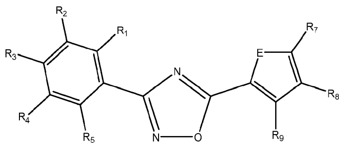
Formula IVa
