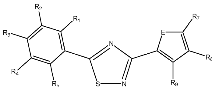
Formula VIIa
