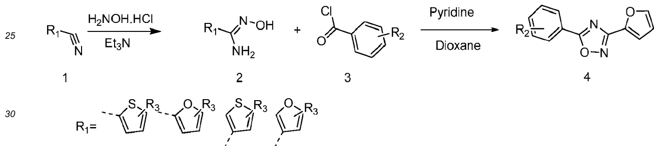
Scheme 5: Synthetic scheme to compounds of the Formula Va and Vb
