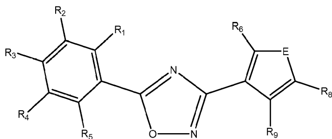
Formula Vb
