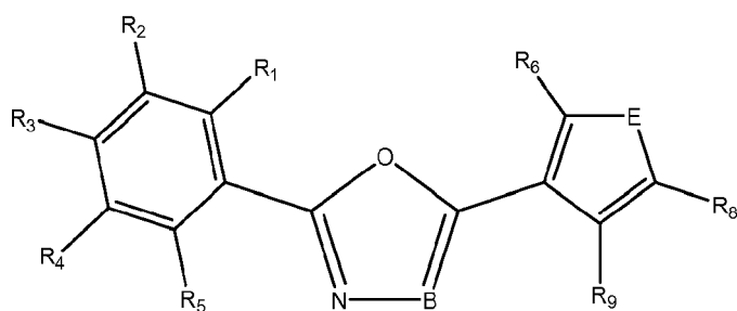
Formula IIb
