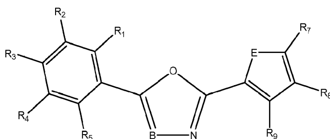
Formula Ia
