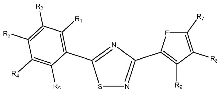
Formula VIIa
