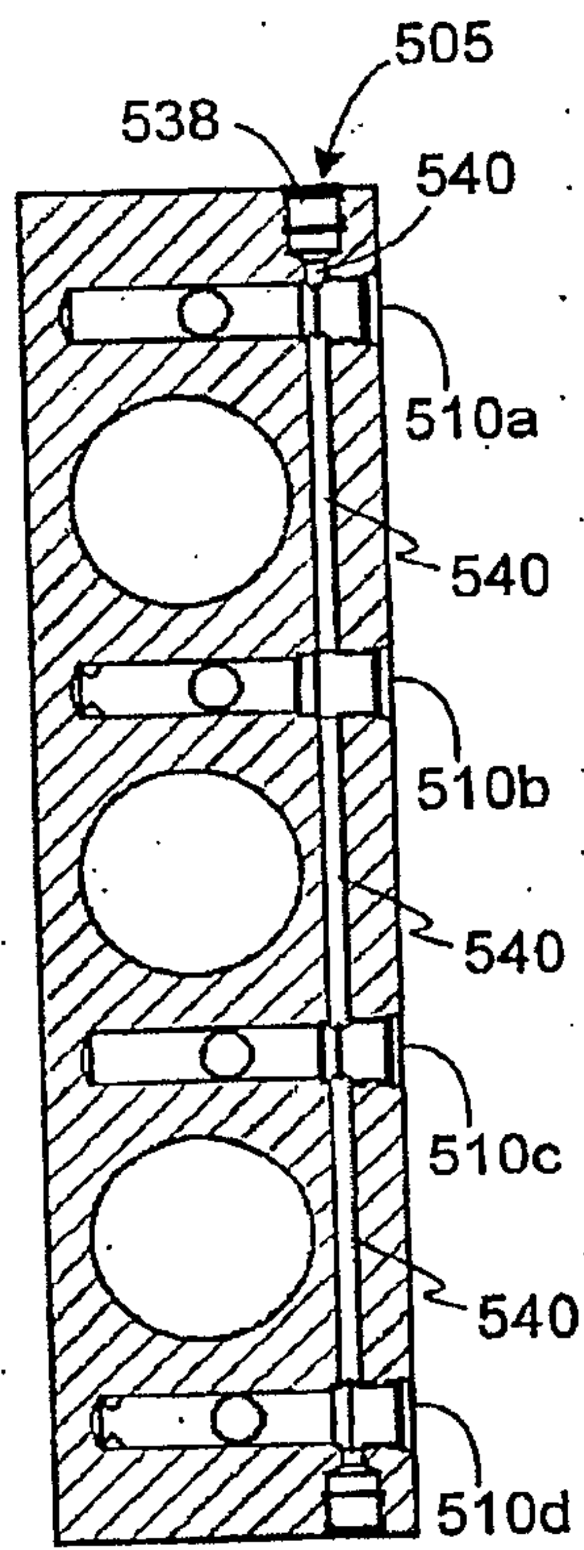
SECTION C-C FIG. 10C
