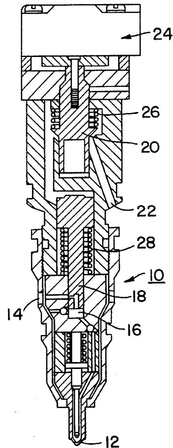
FIG. 2 PRIOR ART
