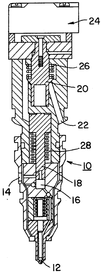
FIG. 1 PRIOR ART
