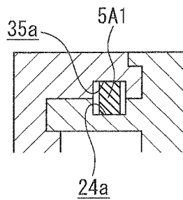
(c) CROSS-SECTION ALONG B-B
