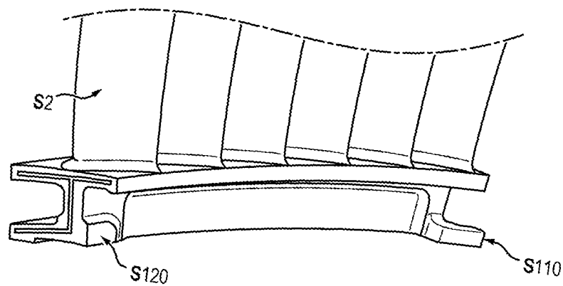
FIG. 2 Prior Art
