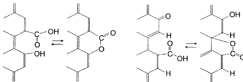
(b) lactonic carboxyl group (and lactone group)
