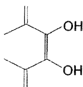
(c) phenolic hydroxyl group
