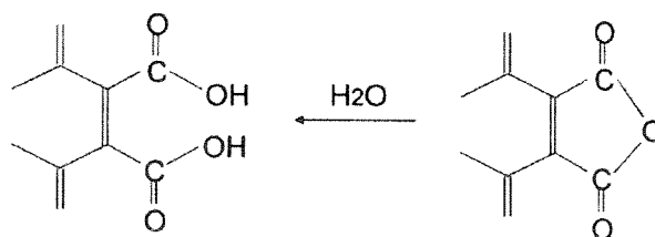
(a) carboxyl group (and anhydrous carboxyl group)
