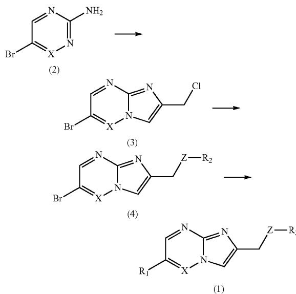
[Reaction Scheme 1]
