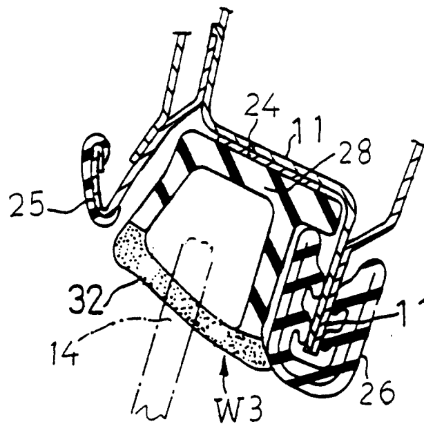
FIG. 4 (PRIOR ART)
