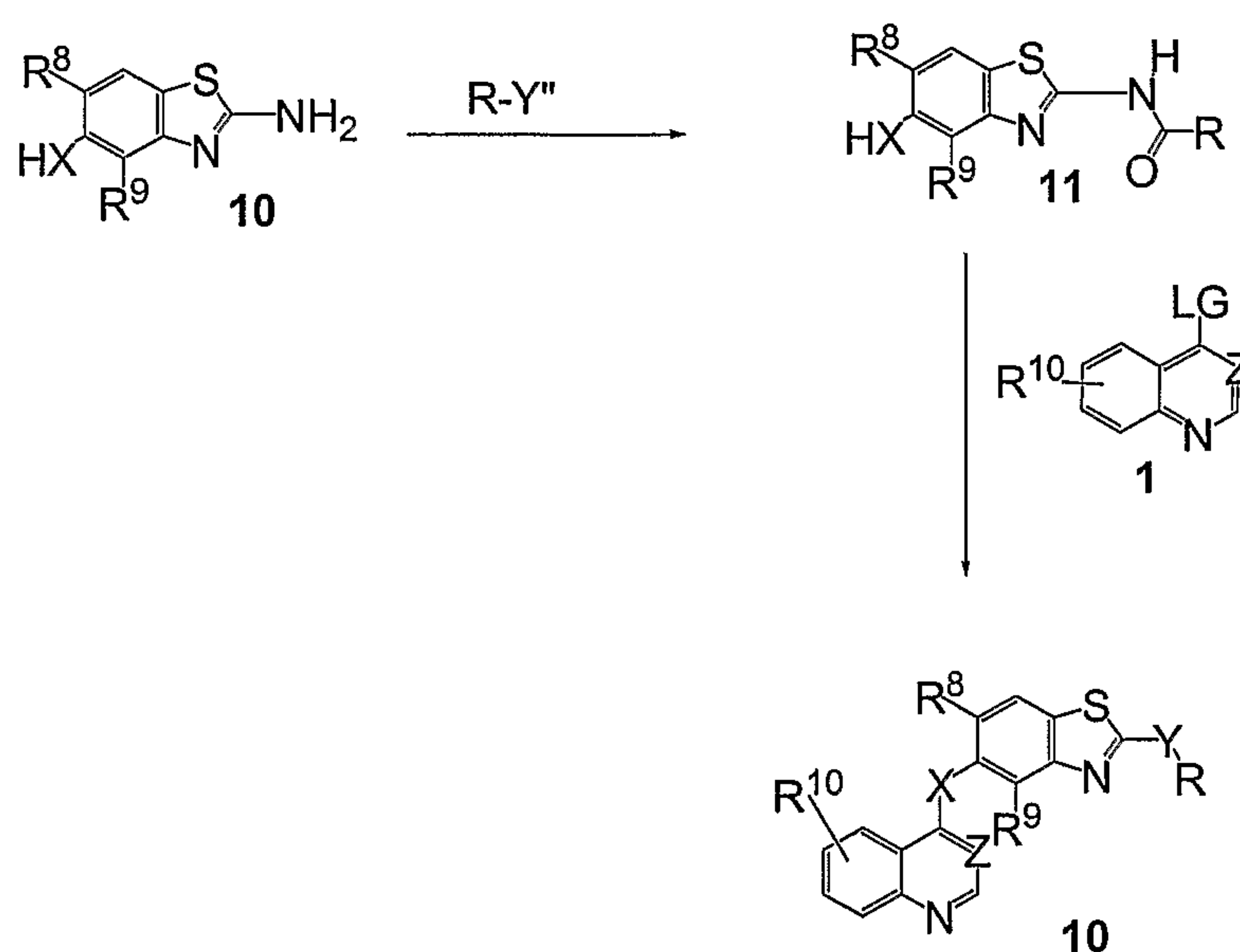
Scheme 5
