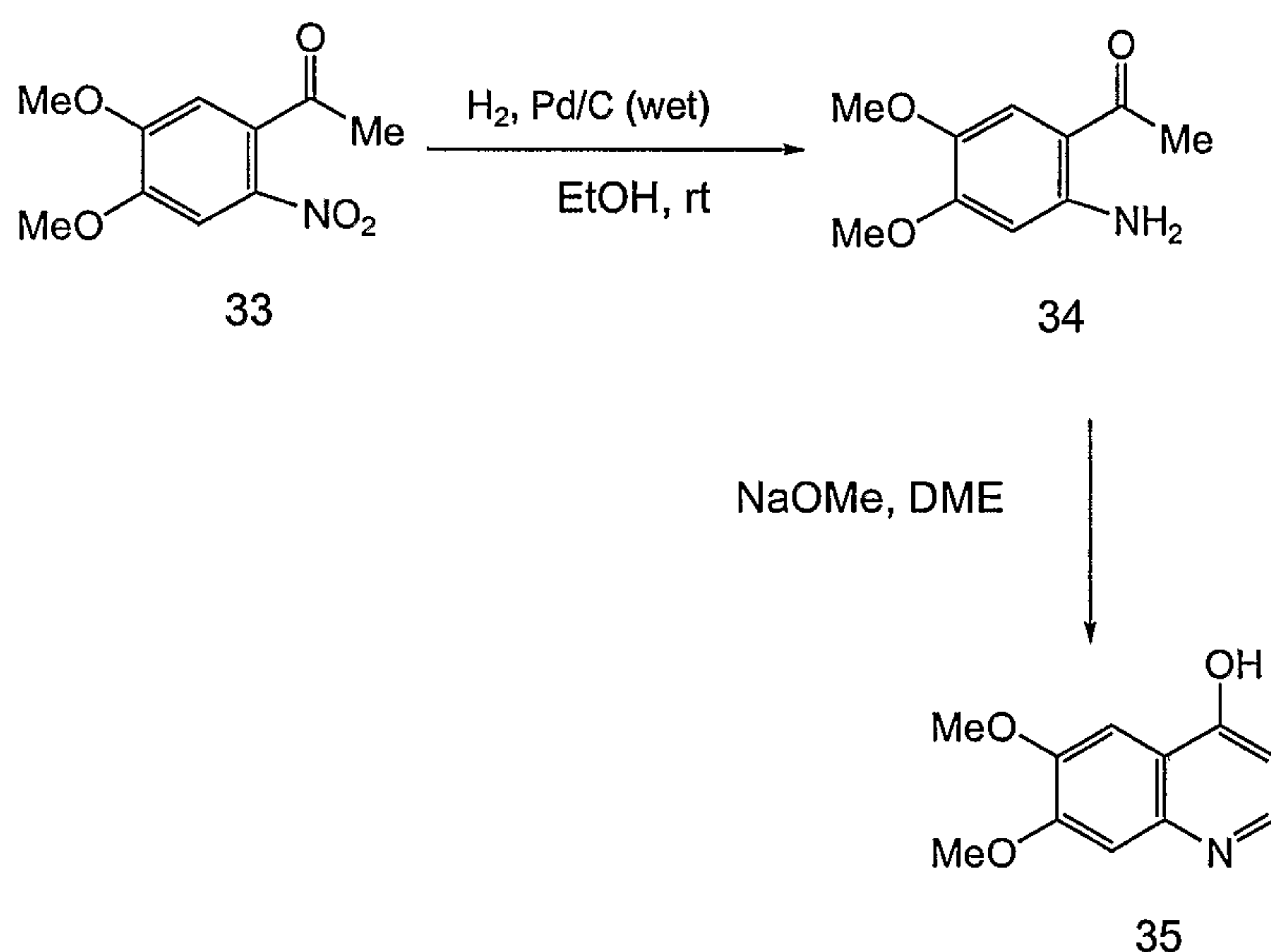
Scheme 13
