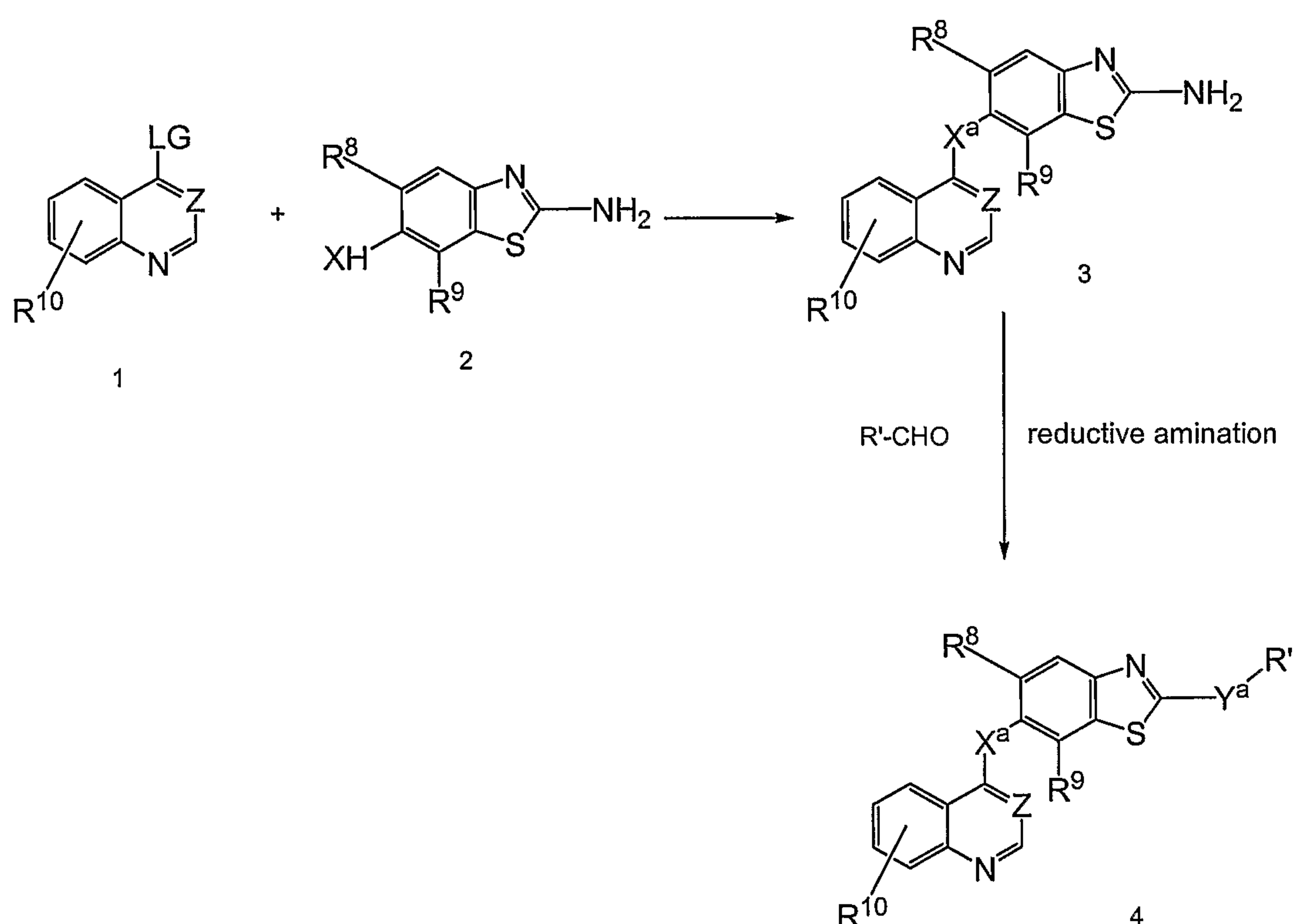
Scheme 1
