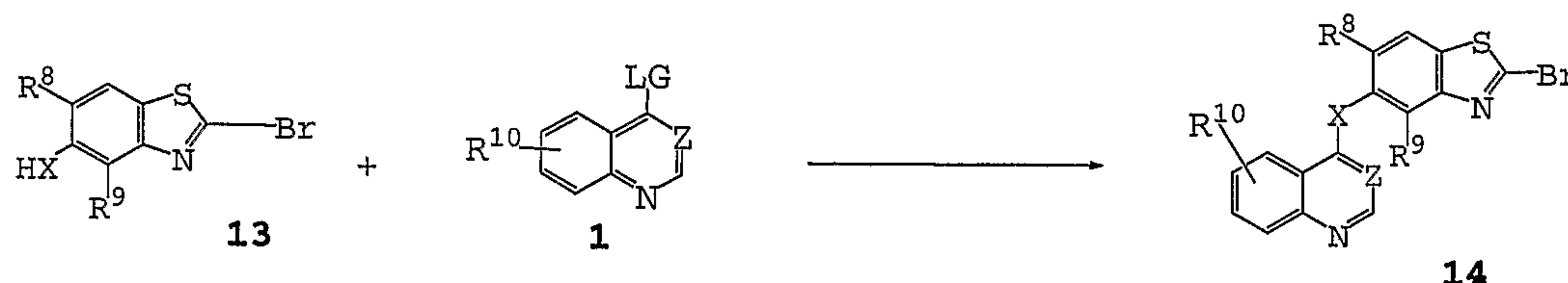
Scheme 6
