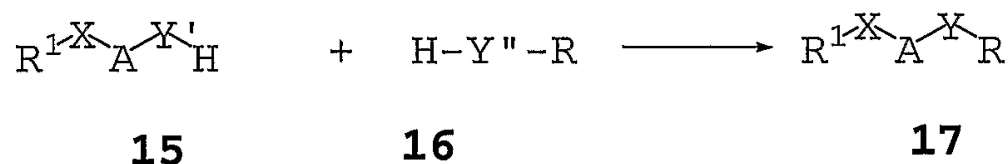
Scheme 7
