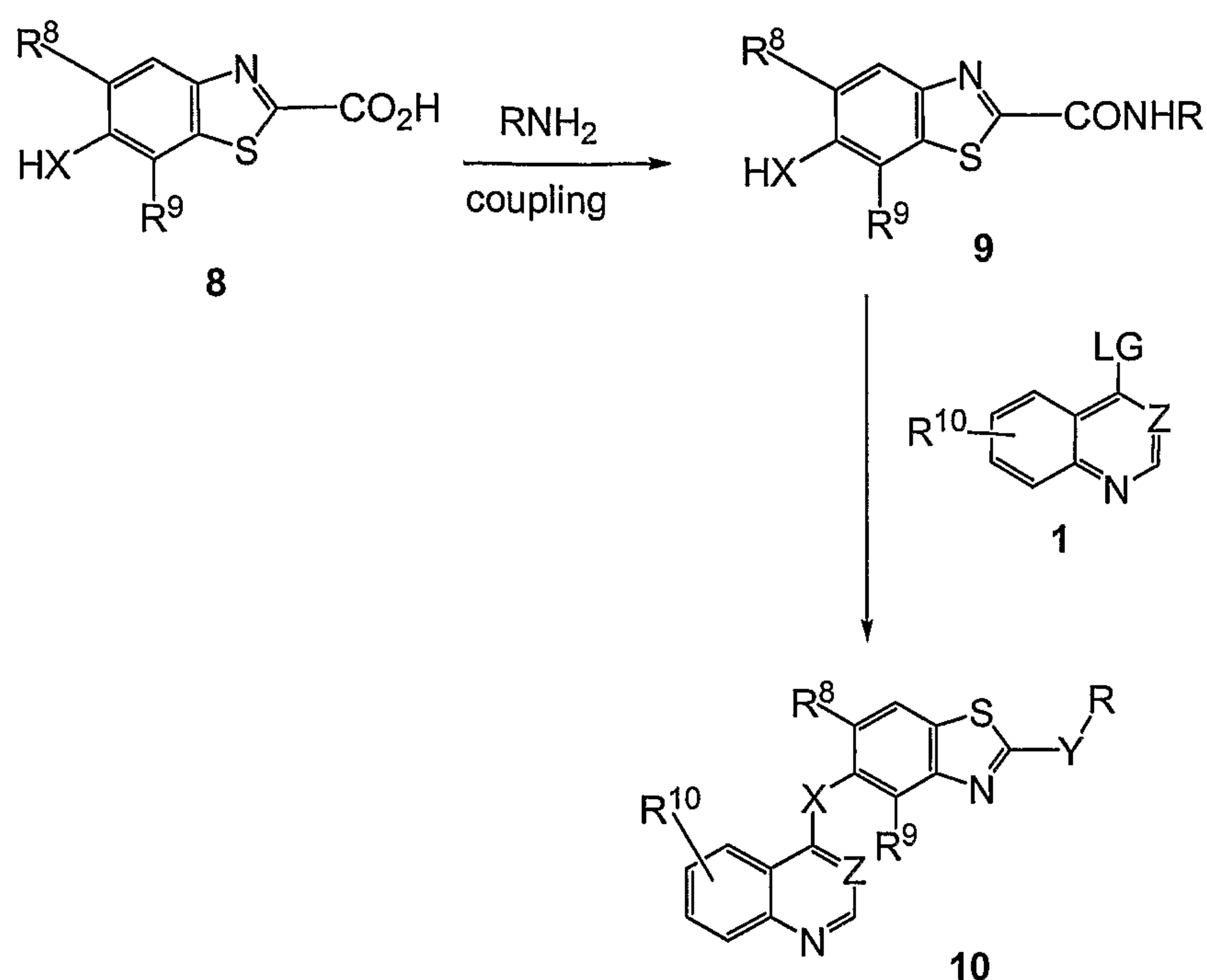
Scheme 4
