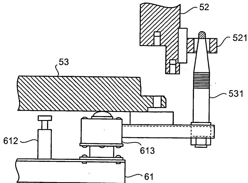
ENLARGED VIEW OF J PORTION
