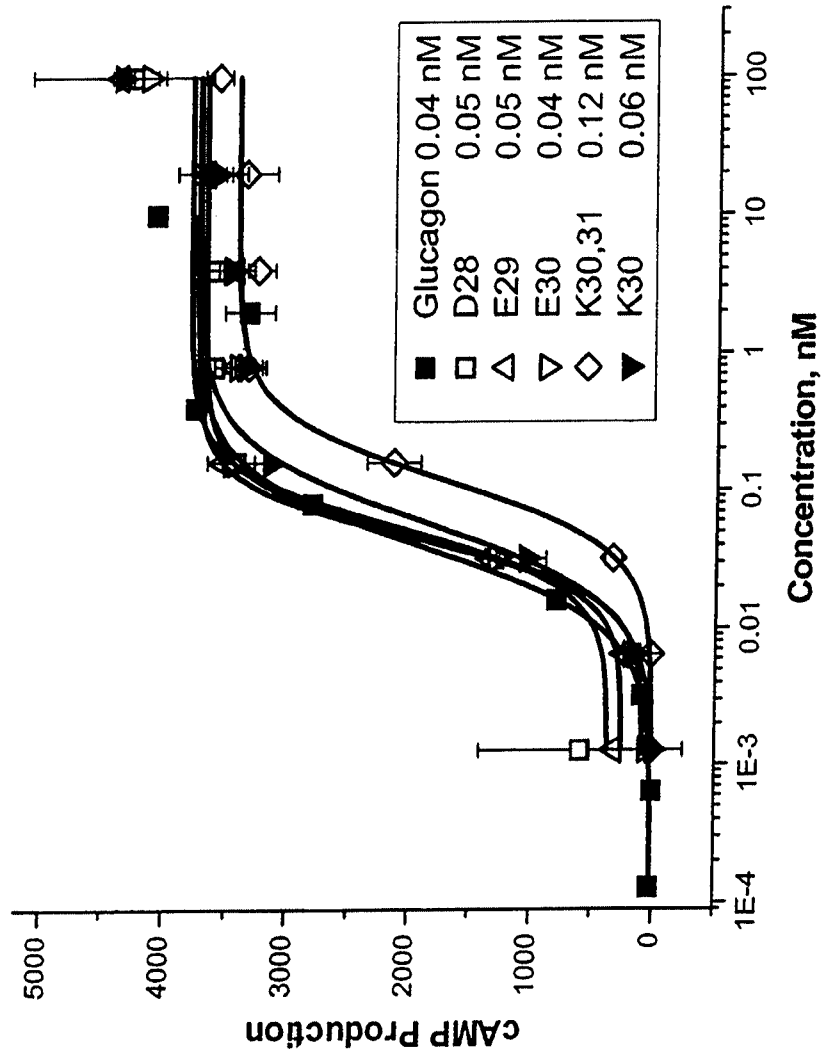
Fig. 7 Glucagon Receptor-mediated cAMP Induction
