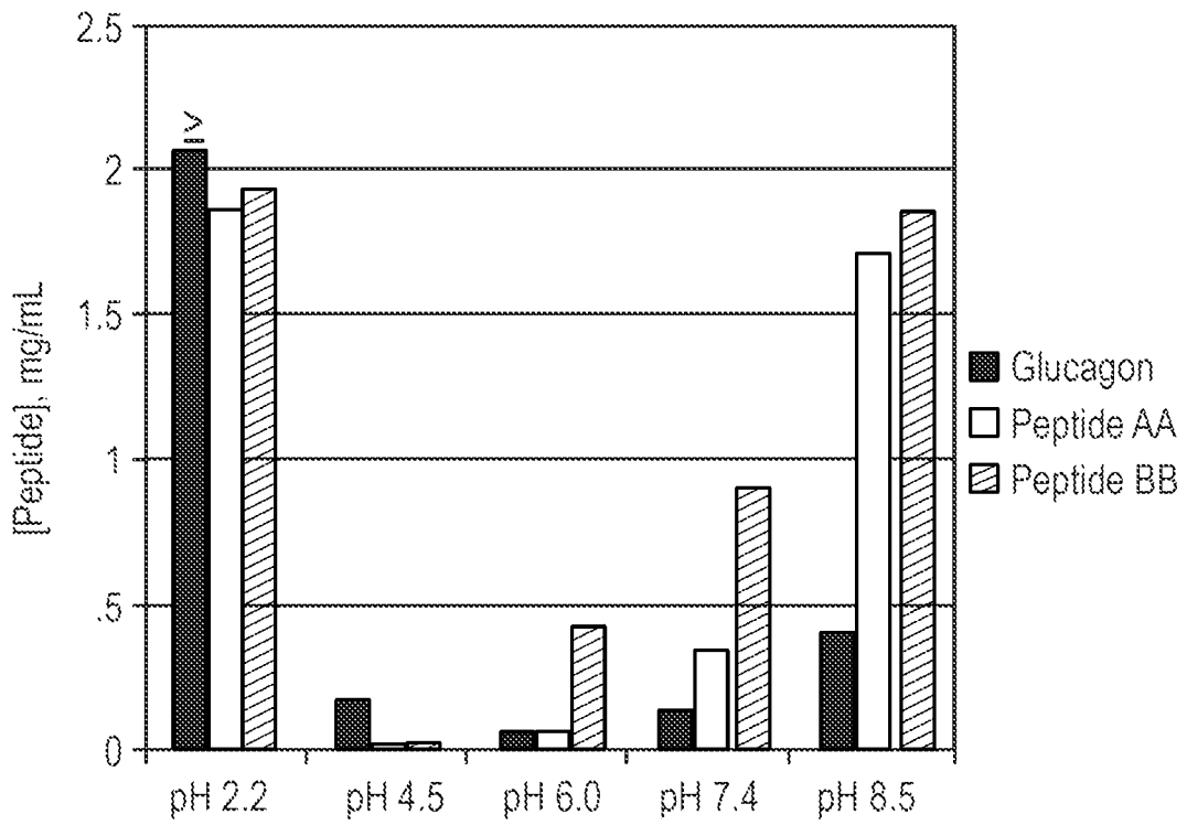
Maximum Solubility of Stabilized Glucagon Analogs at Various pH Values
