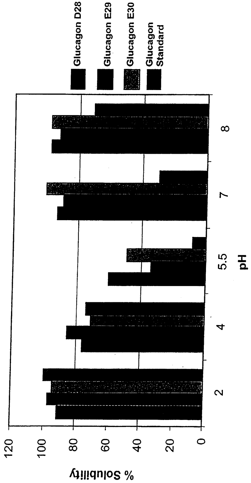
Fig. 3 Solubility and Stability of Glucagon Analogs after 60 hrs at 25°C at Various pHs
