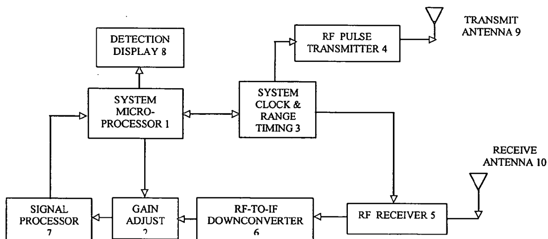
Figure 2. Pattern Shaping Gain Adjustment in Signal Processor Section
