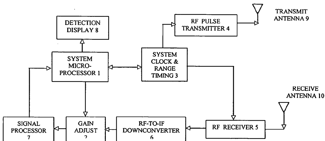
Pattern Shaping Gain Adjustment in Signal Processor Section
