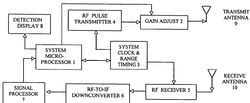
Figure 1C. Pattern Shaping Gain Adjustment Made in Transmitter Section
