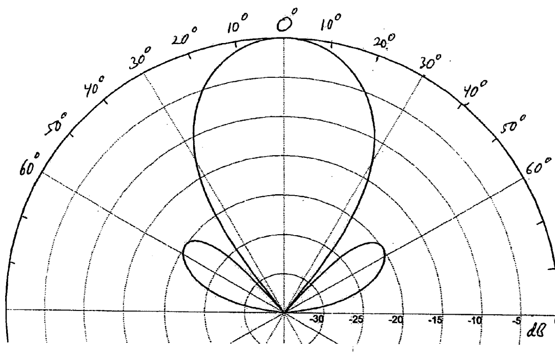
Figure 4. Typical Antenna Power Pattern Polar Plot
