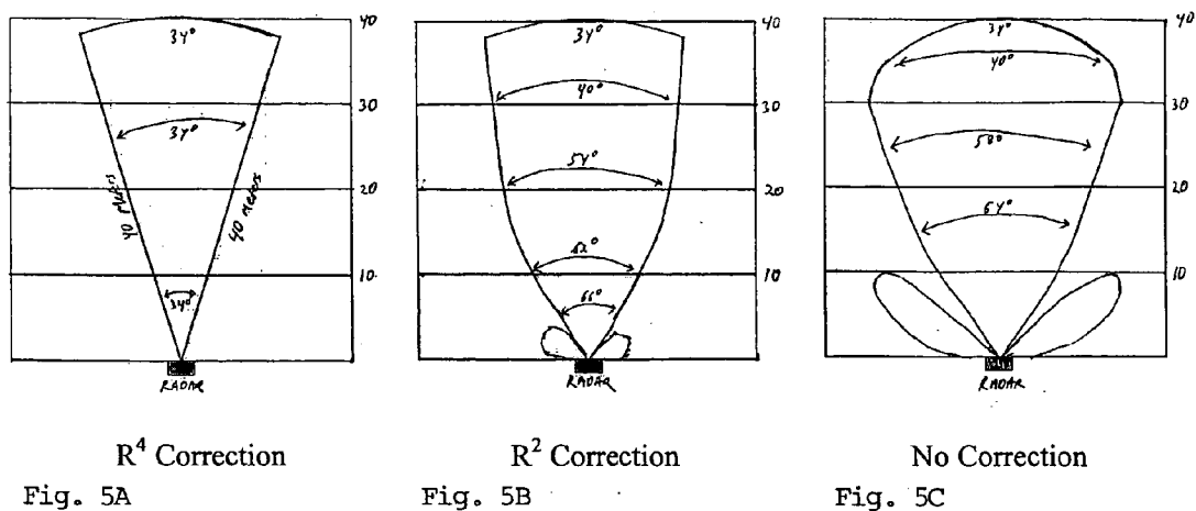
Figure 5. Typical Radar Detection Coverage Areas Corresponding To Fixed Range-Dependent Gain Correction
