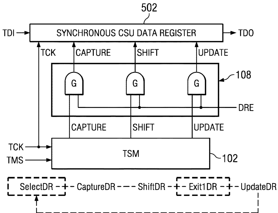
FIG. 5 (PRIOR ART)
