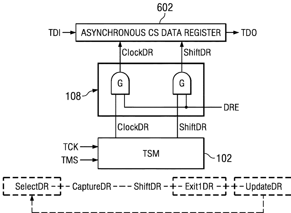
FIG. 6 (PRIOR ART)
