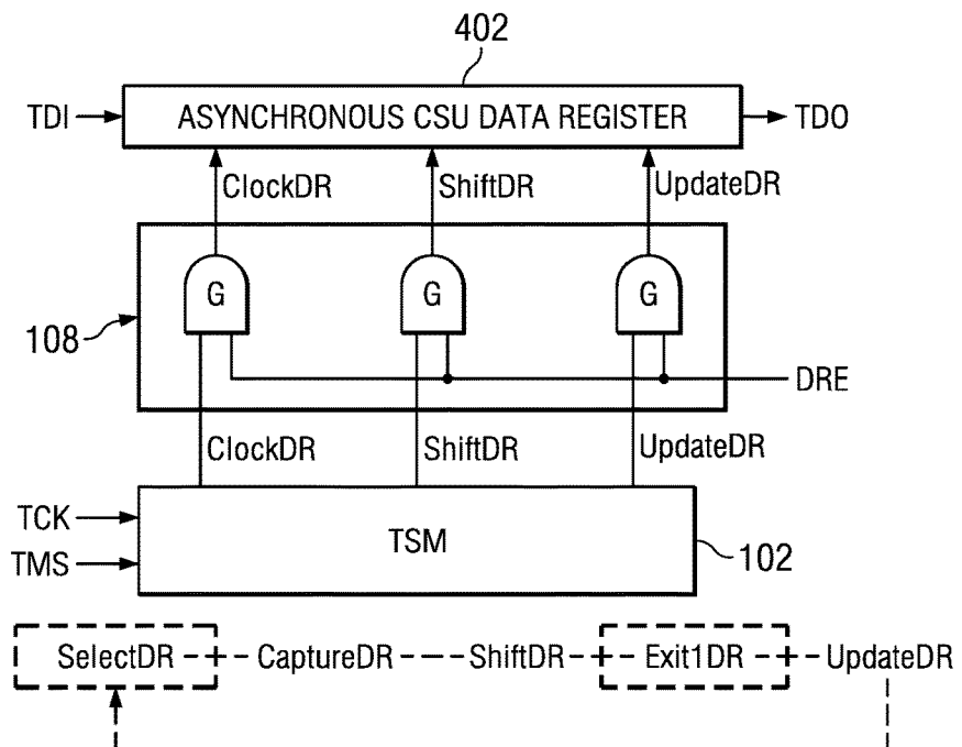
FIG. 4 (PRIOR ART)
