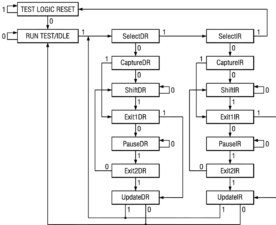
FIG. 3 (PRIOR ART)
