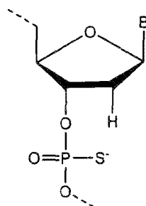
Phosphorothioate DNA Unit (PS) Structure 1
