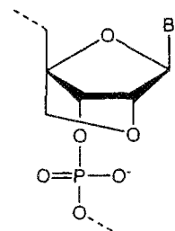
Locked nucleic acid unit (LNA) Structure 5
