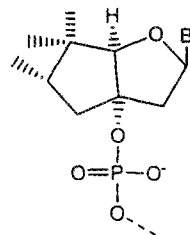
Tricyclonucleic acid unit Structure 9
