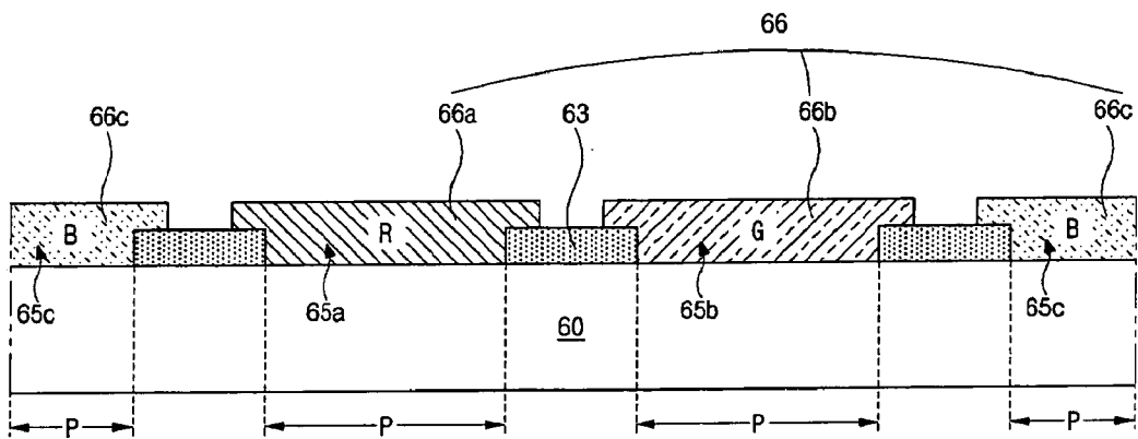
FIG. 2C (related art)
