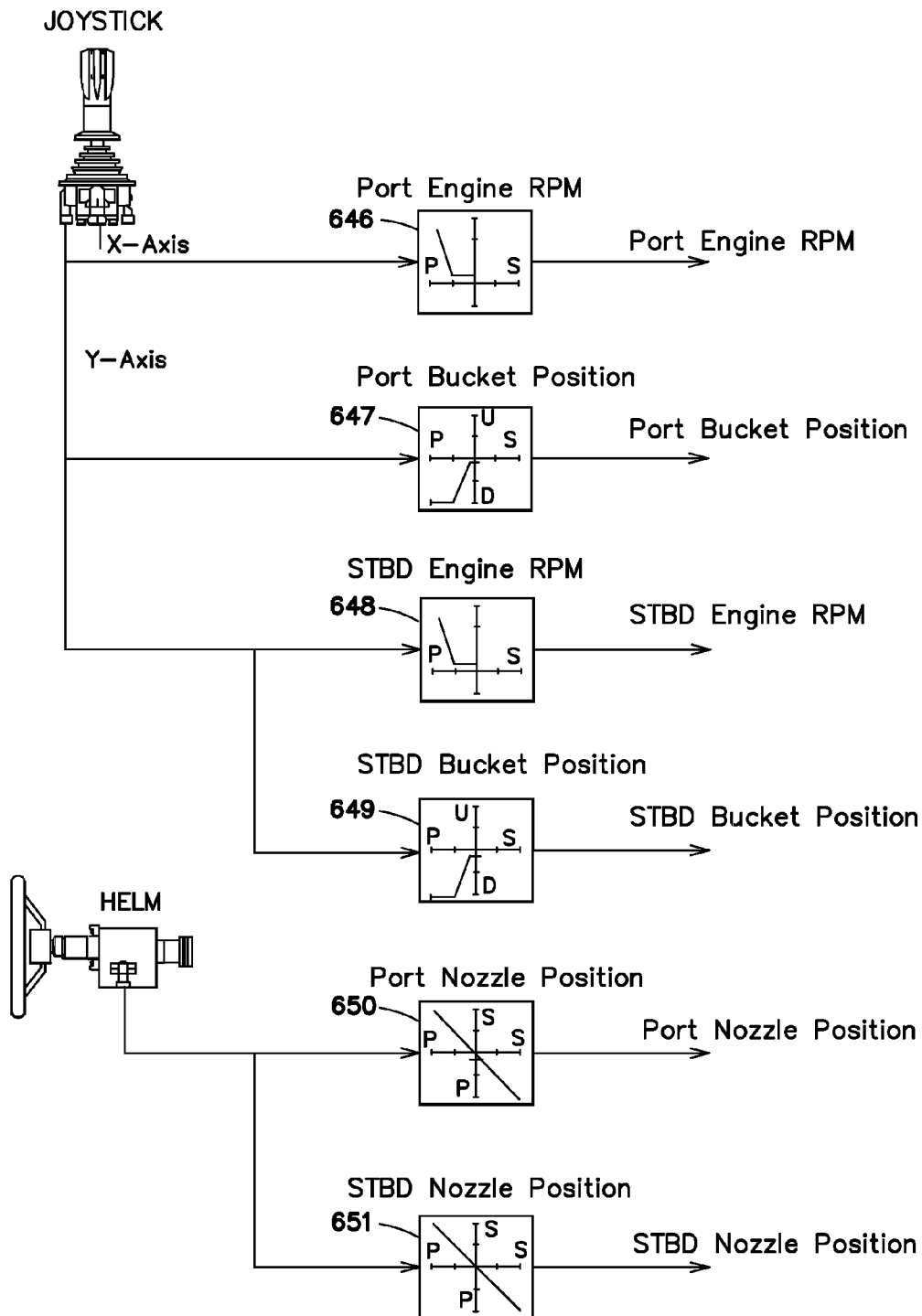
Integrated Twin Waterjet Signal Diagram: Zone 5 (Thrust AST Only )
