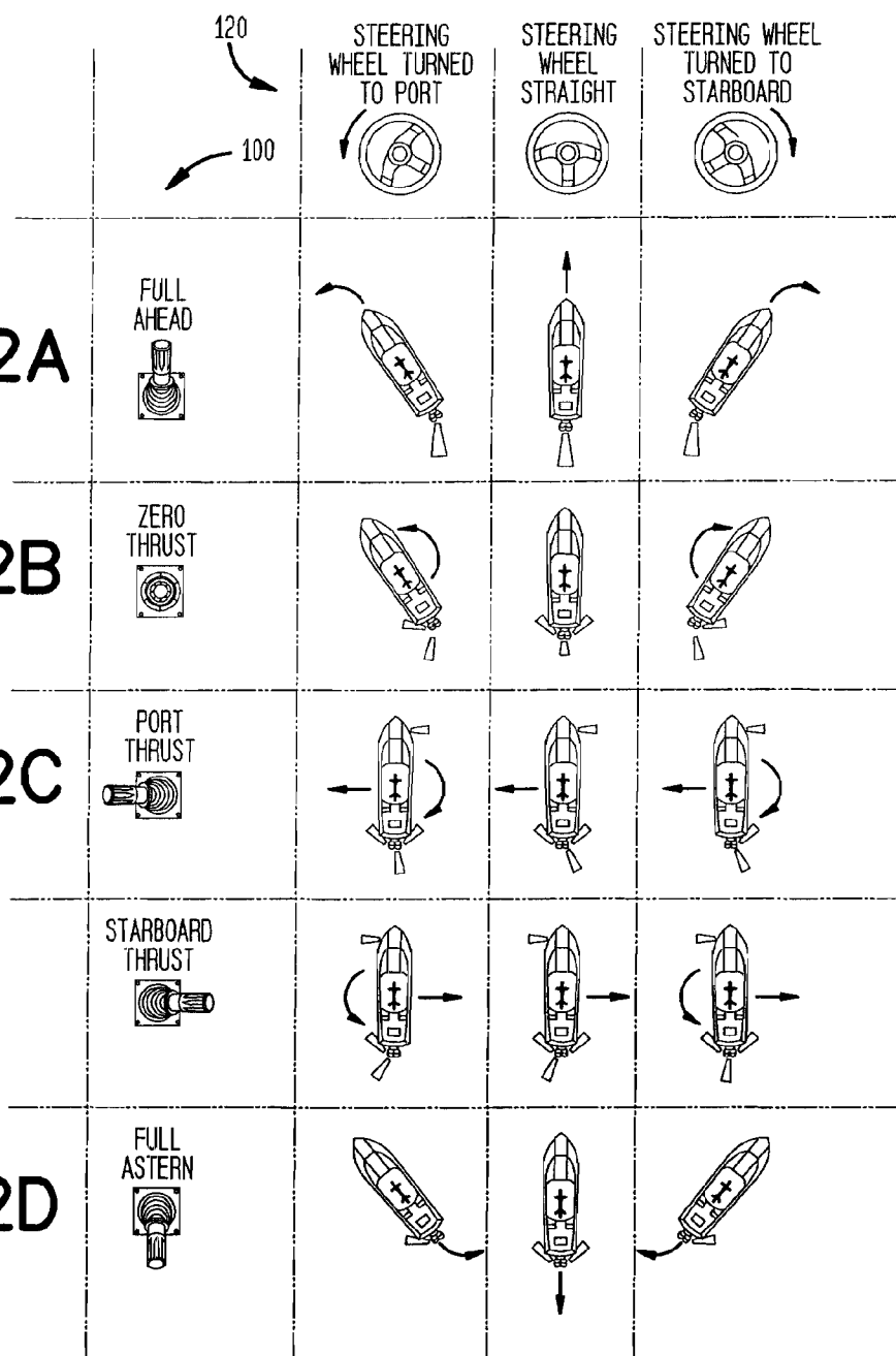
SINGLE WATERJET MOTION DIAGRAM
