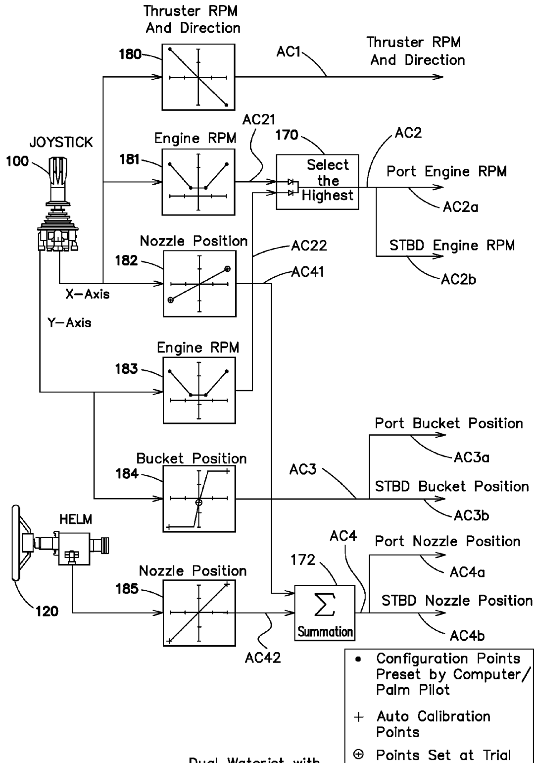
Dual Waterjet with Bow Thruster Signal Diagram
