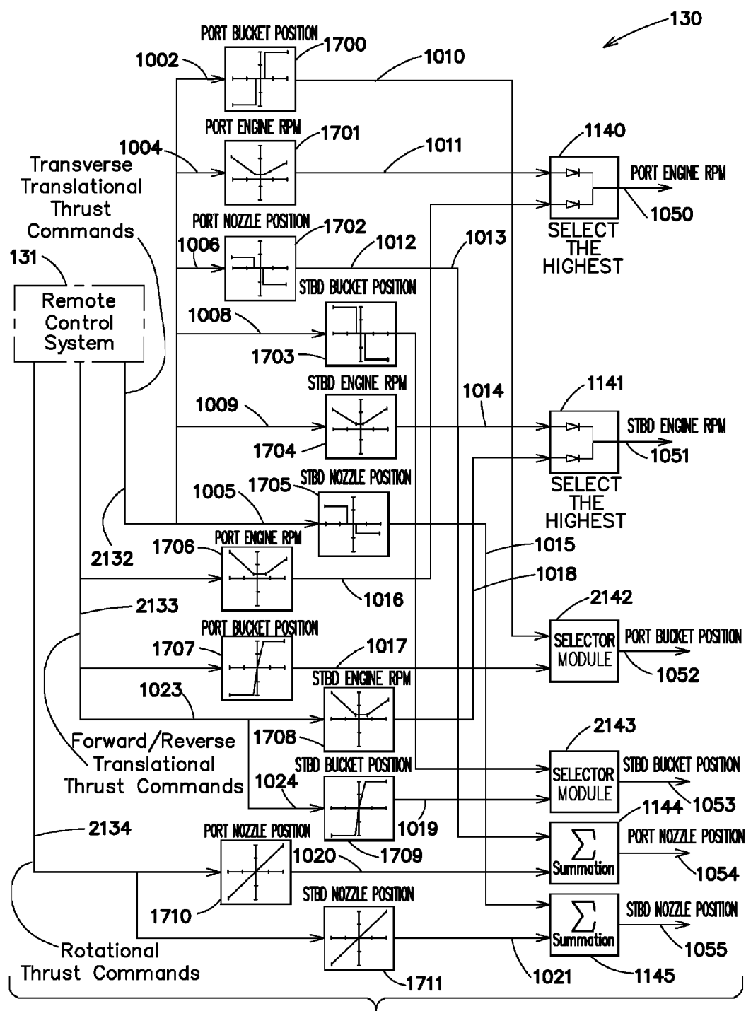
TWIN WATERJET SIGNAL DIAGRAM REMOTELY CONTROLLED
