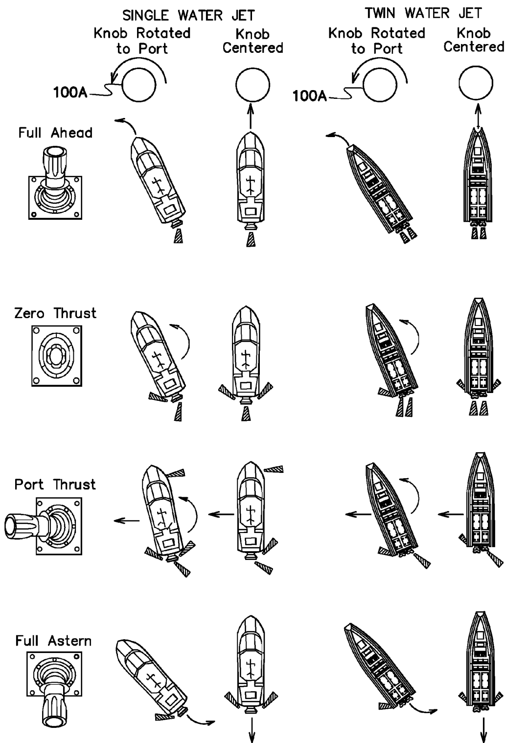
Three-Axis Joystick Implementation
