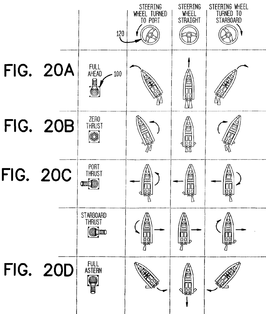
DUAL WATERJET MOTION DIAGRAM
