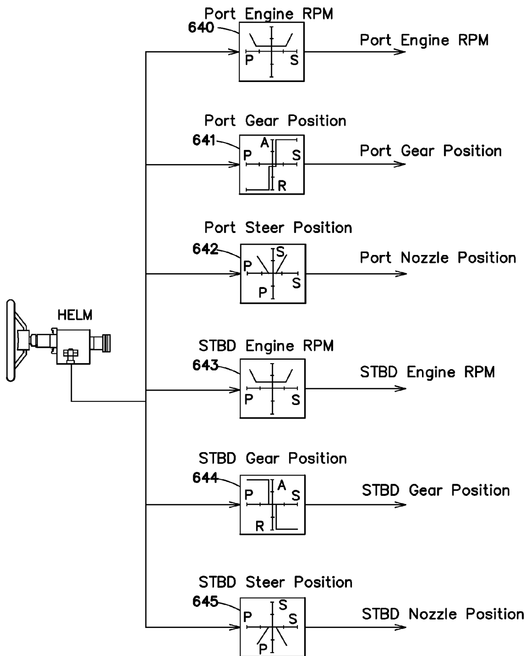
Steerable Propeller Signal Diagram: Zone 3 (Rotation Only (Joystick Centered))
