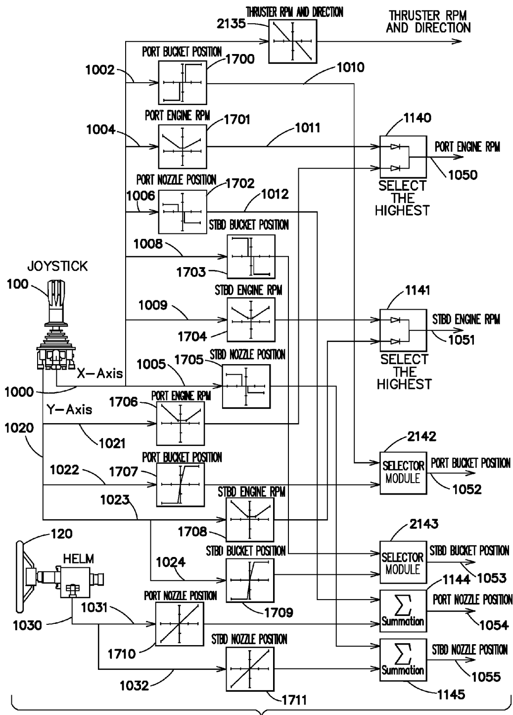
TWIN WATERJET SIGNAL DIAGRAM WITH BOWTHRUSTER
