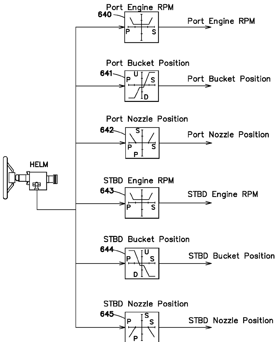
Integrated Twin Waterjet Signal Diagram: Zone 3 (Rotation Only (Joystick Centered))
