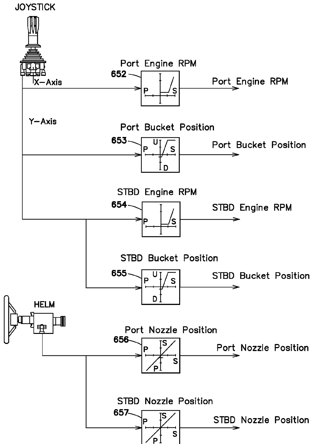
Integrated Twin Waterjet Signal Diagram: Zone 4 (Thrust AHD Only )
