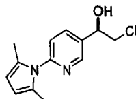
(1R)-2-Chloro-1-[6-(2,5-dimethyl-pyrrol-1-yl)-pyridin-3-yl]-ethanol
