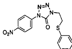
1-(4-Nitrophenyl)-4-(2-phenylsulfanylethyl)-1,4-dihydrotetrazol-5-one
