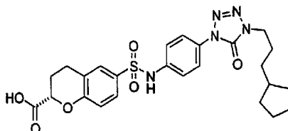
6-{4-[4-(3-Cyclopentyl-propyl)-5-oxo-4,5-dihydro-tetrazol-1-yl]-phenylsulfamoyl}-chroman-(S)-2-carboxylic acid
