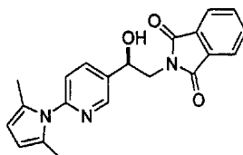
20 (R)-2-[2-[6-(2,5-Dimethylpyrrol-1-yl)pyridin-3-yl]-2-hydroxyethyl]isoindol-1,3-dione
