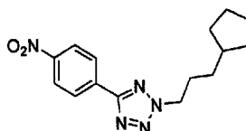
2-(3-Cyclopentyl-propyl)-5-(4-nitro-phenyl)-2N-tetrazole
