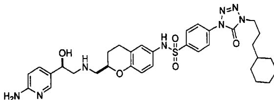
N-((2R)-2-(((2R)-2-(6-Amino-pyridin-3-yl)-2-hydroxy-ethylamino)-methyl)-chroman-6-yl)-4-[4-(3-cyclohexyl-propyl)-5-oxo-4,5-dihydro-tetrazol-1-yl]-benzenesulfonamide
