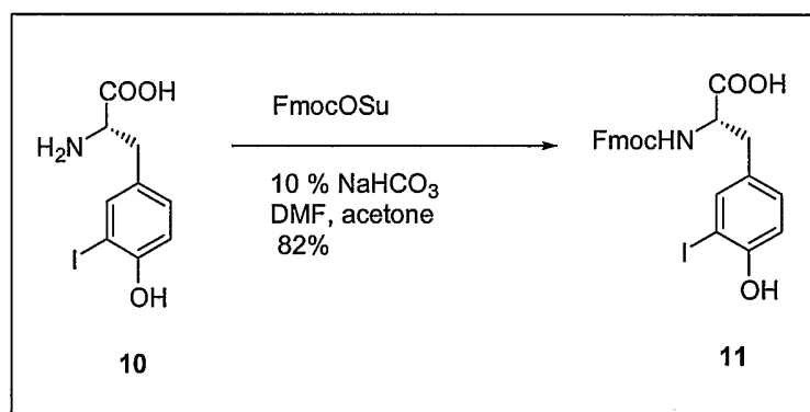
Scheme 1: Synthesis of Fmoc-(3-I)-Tyr-OH, 11
