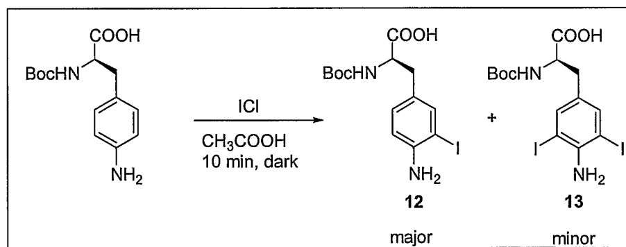
Scheme 2: Synthesis of Boc-(4-amino-3-iodo)-D-Phe-OH, 12
