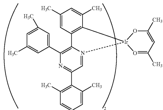
[\text{Ir}(\text{dmdppr-dmp})_2(\text{acac})]
