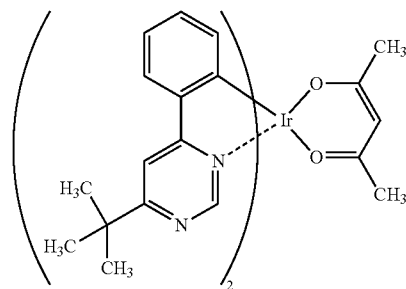
[\text{Ir}(\text{tBuppm})_2(\text{acac})]
