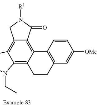
Scheme 15.
