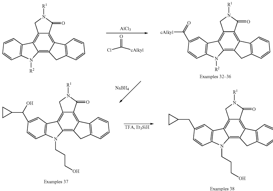
Scheme 7.
