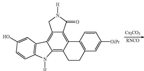
Intermediate I-14
