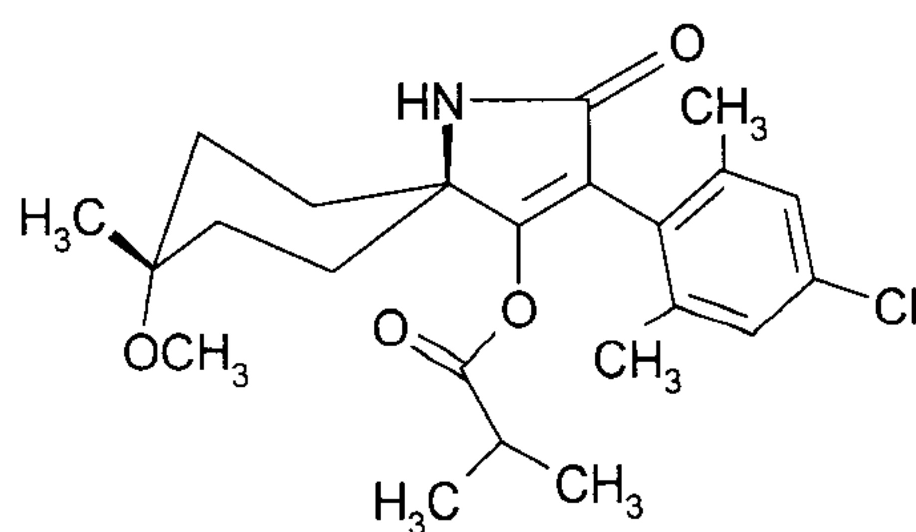
trans α-Isomer
