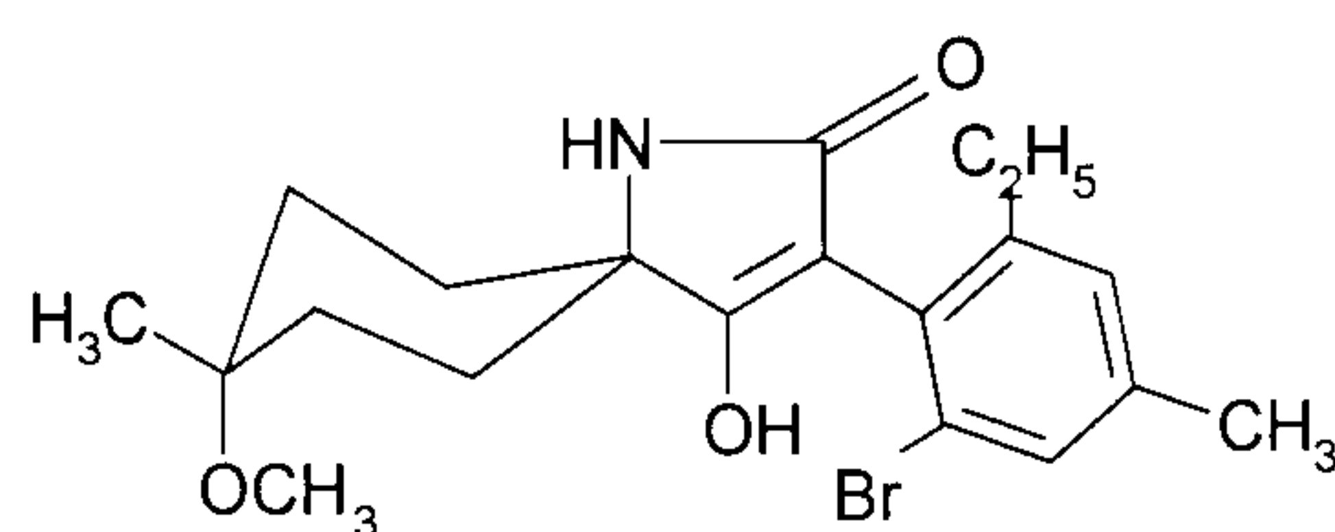
I-a-1
