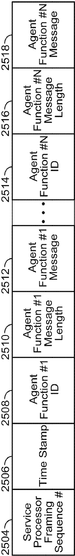
28/106 Service Processor Communication Frame 2502
