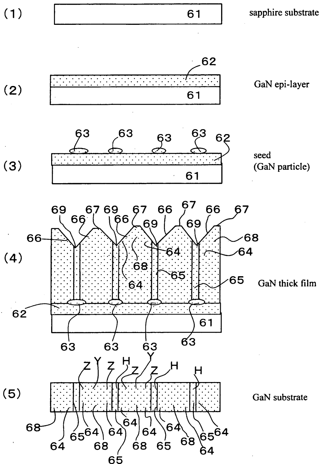
Fig.13 Embodiment 4 Processes of producing a GaN substrate
