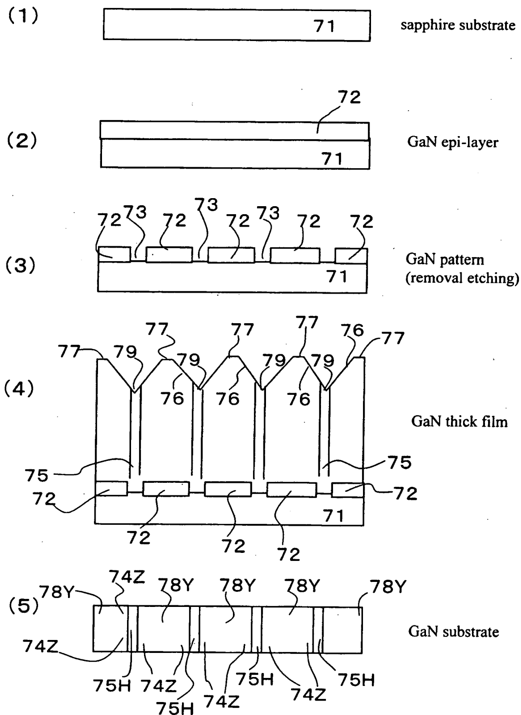
Fig.14 Processes of producing a GaN substrate
