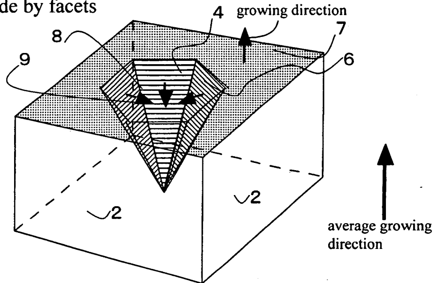
Fig.1 Prior Art decrement of dislocations by a pit made by facets
