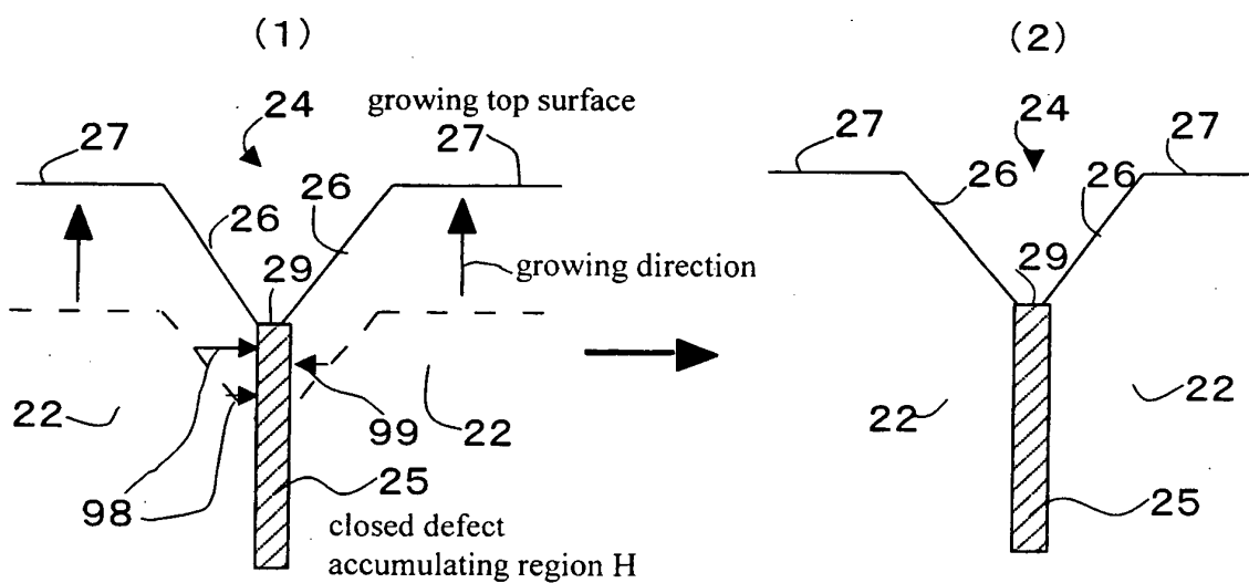
Fig.4 growing method of the present invention
