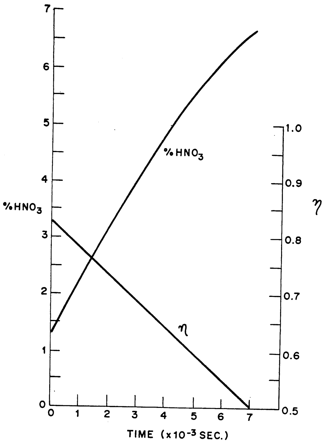
FIG. 3 GENERATION OF \text{HNO}_3 FROM \text{KNO}_3
