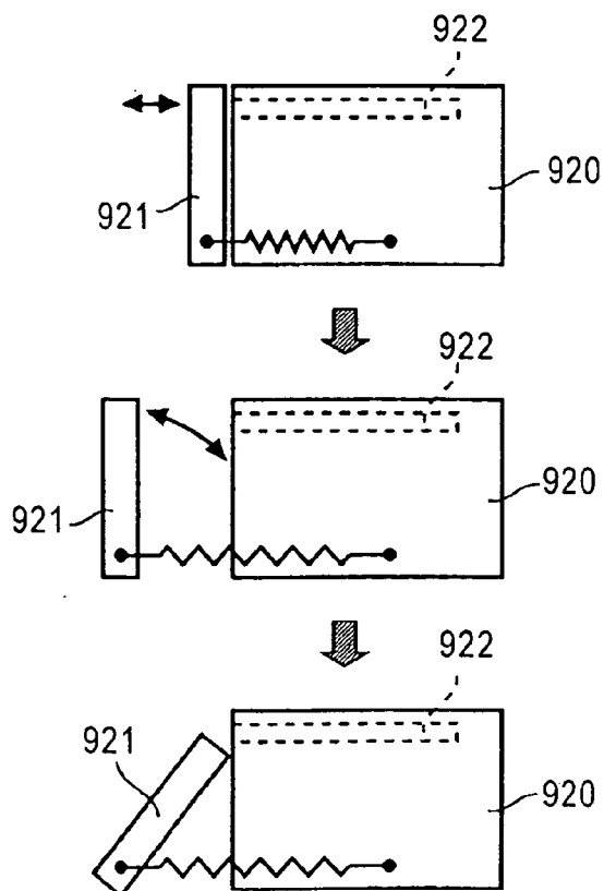
FIG. 13C PRIOR ART
