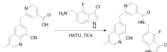
N-((3-chloro-4-fluoro-1H-indol-5-yl)methyl)-2-((8-cyano-3-methylquinolin-6-yl)methyl)isonicotinamide
