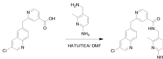
N -(6-Amino-2-methyl-pyridin-3-ylmethyl)-2-(3-chloro-quinolin-6-ylmethyl)-isonicotinamide
