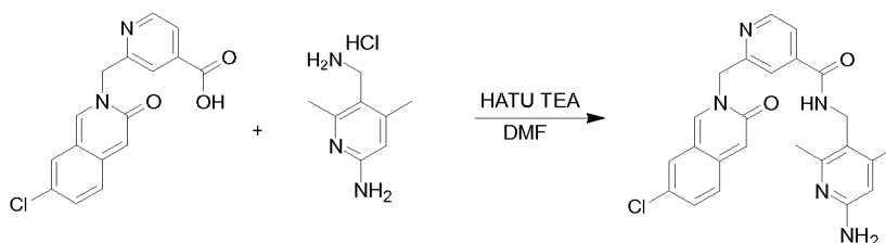
N-((6-amino-2,4-dimethylpyridin-3-yl)methyl)-2-((7-chloro-3-oxoisoquinolin-2(3H)-yl)methyl)isonicotinamide
