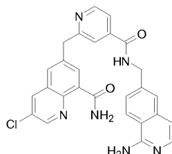
6-((4-(((1-aminoisoquinolin-6-yl)methyl)carbamoyl)pyridin-2-yl)methyl)-3-chloroquinoline-8-carboxamide
