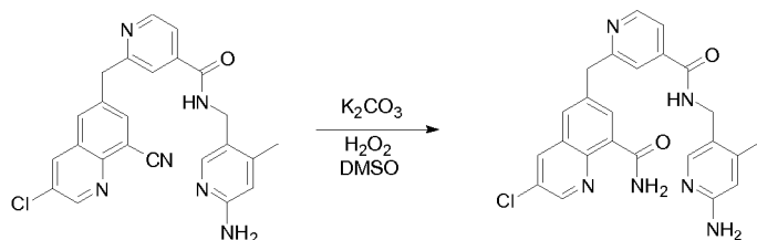
6-((4-(((6-amino-4-methylpyridin-3-yl)methyl)carbamoyl)pyridin-2-yl)methyl)-3-chloroquinoline-8-carboxamide
