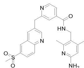
N -((6-amino-2,4-dimethylpyridin-3-yl)methyl)-2-((6-(methylsulfonyl)quinolin-3-yl)methyl)isonicotinamide
