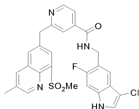
N-((3-chloro-6-fluoro-1H-indol-5-yl)methyl)-2-((3-methyl-8-(methylsulfonyl)quinolin-6-yl)methyl)isonicotinamide
