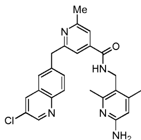
N -((6-amino-2,4-dimethylpyridin-3-yl)methyl)-2-((3-chloroquinolin-6-yl)methyl)-6-methylisonicotinamide
