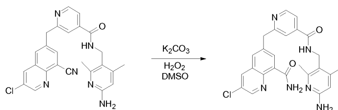
6-((4-(((6-amino-2,4-dimethylpyridin-3-yl)methyl)carbamoyl)pyridin-2-yl)methyl)-3-chloroquinoline-8-carboxamide
