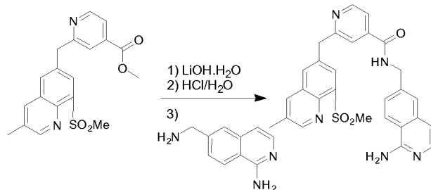
N-((1-aminoisoquinolin-6-yl)methyl)-2-((3-methyl-8-(methylsulfonyl)quinolin-6-yl)methyl)isonicotinamide
