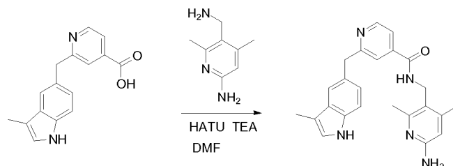
N -((6-amino-2,4-dimethylpyridin-3-yl)methyl)-2-((3-methyl-1 H -indol-5-yl)methyl)isonicotinamide
