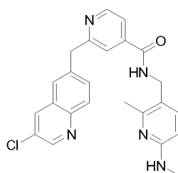
2-((3-chloroquinolin-6-yl)methyl)-N-((2-methyl-6-(methylamino)pyridin-3-yl)methyl)isonicotinamide
