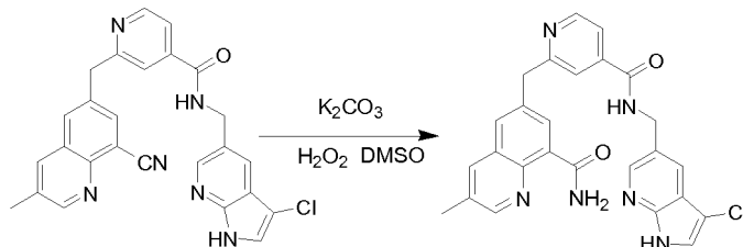
6-((4-(((3-chloro-1H-pyrrolo[2,3-b]pyridin-5-yl)methyl)carbamoyl)pyridin-2-yl)methyl)-3-methylquinoline-8-carboxamide
