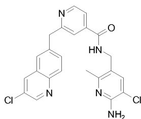
N-((6-amino-5-chloro-2-methylpyridin-3-yl)methyl)-2-((3-chloroquinolin-6-yl)methyl)isonicotinamide
