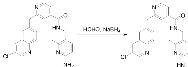
2-((3-chloroquinolin-6-yl)methyl)-N-((2-methyl-6-(methylamino)pyridin-3-yl)methyl)isonicotinamide
