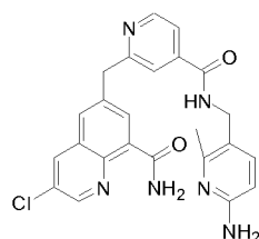
6-((4-(((6-amino-2-methylpyridin-3-yl)methyl)carbamoyl)pyridin-2-yl)methyl)-3-chloroquinoline-8-carboxamide
