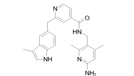
N -((6-amino-2,4-dimethylpyridin-3-yl)methyl)-2-((3-methyl-1 H -indol-5-yl)methyl)isonicotinamide
