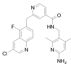
N-((6-amino-2,4-dimethylpyridin-3-yl)methyl)-2-((3-chloro-5-fluoroquinolin-6-yl)methyl)isonicotinamide
