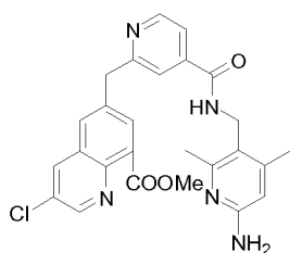
methyl 6-((4-(((6-amino-2,4-dimethylpyridin-3-yl)methyl)carbamoyl)pyridin-2-yl)methyl)-3-chloroquinoline-8-carboxylate
