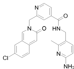
N-((6-amino-2-methylpyridin-3-yl)methyl)-2-((7-chloro-3-oxoisoquinolin-2(3H)-yl)methyl)isonicotinamide
