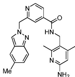
N -((6-amino-2,4-dimethylpyridin-3-yl)methyl)-2-((5-methyl-2 H -indazol-2-yl)methyl)isonicotinamide
