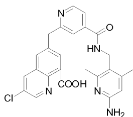
6-((4-(((6-amino-2,4-dimethylpyridin-3-yl)methyl)carbamoyl)pyridin-2-yl)methyl)-3-chloroquinoline-8-carboxylic acid
