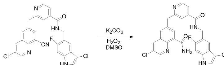
3-chloro-6-((4-(((3-chloro-6-fluoro-1H-indol-5-yl)methyl)carbamoyl)pyridin-2-yl)methyl)quinoline-8-carboxamide
