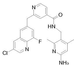
N-(6-Amino-2,4-dimethyl-pyridin-3-ylmethyl)-2-(3-chloro-8-fluoro-quinolin-6-ylmethyl)-isonicotinamide
