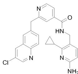
N-((6-amino-2-cyclopropylpyridin-3-yl)methyl)-2-((3-chloroquinolin-6-yl)methyl)isonicotinamide
