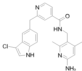
N -((6-amino-2,4-dimethylpyridin-3-yl)methyl)-2-((3-chloro-1 H -indol-5-yl)methyl)isonicotinamide
