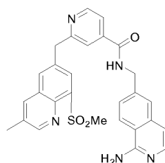
N-((1-aminoisoquinolin-6-yl)methyl)-2-((3-methyl-8-(methylsulfonyl)quinolin-6-yl)methyl)isonicotinamide
