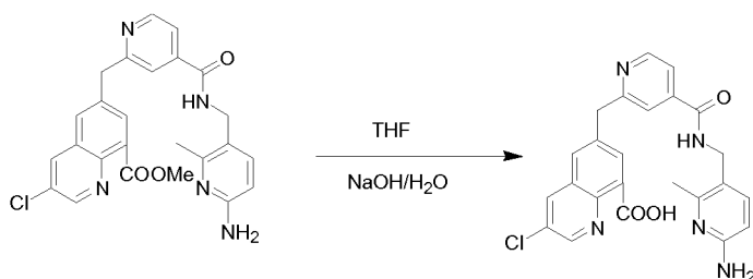
6-((4-(((6-amino-2-methylpyridin-3-yl)methyl)carbamoyl)pyridin-2-yl)methyl)-3-chloroquinoline-8-carboxylic acid
