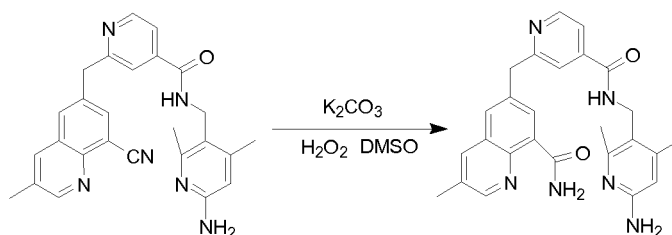
6-((4-(((6-amino-2,4-dimethylpyridin-3-yl)methyl)carbamoyl)pyridin-2-yl)methyl)-3-methylquinoline-8-carboxamide
