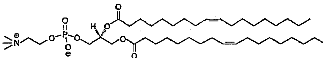
1,2-Dioleoyl-sn-glycero-3-phosphatidylcholine (DOPC)
