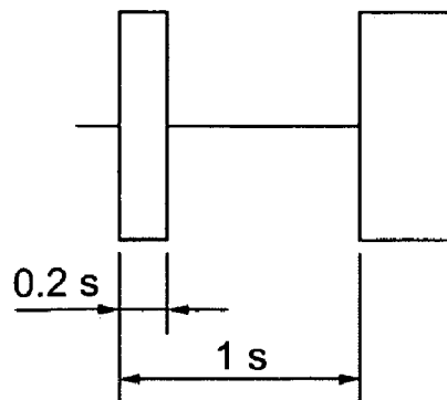
P SIGNAL
