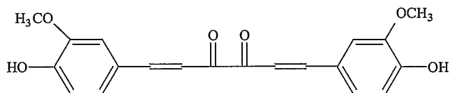
curcumin (7 -Bis (4 -hydroxy -3-methoxyphenyl) -1,6 -heptadiene -3,5 -dione)
