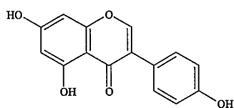
genistein (4',5,7 -trihydroxy -isoflavone)
