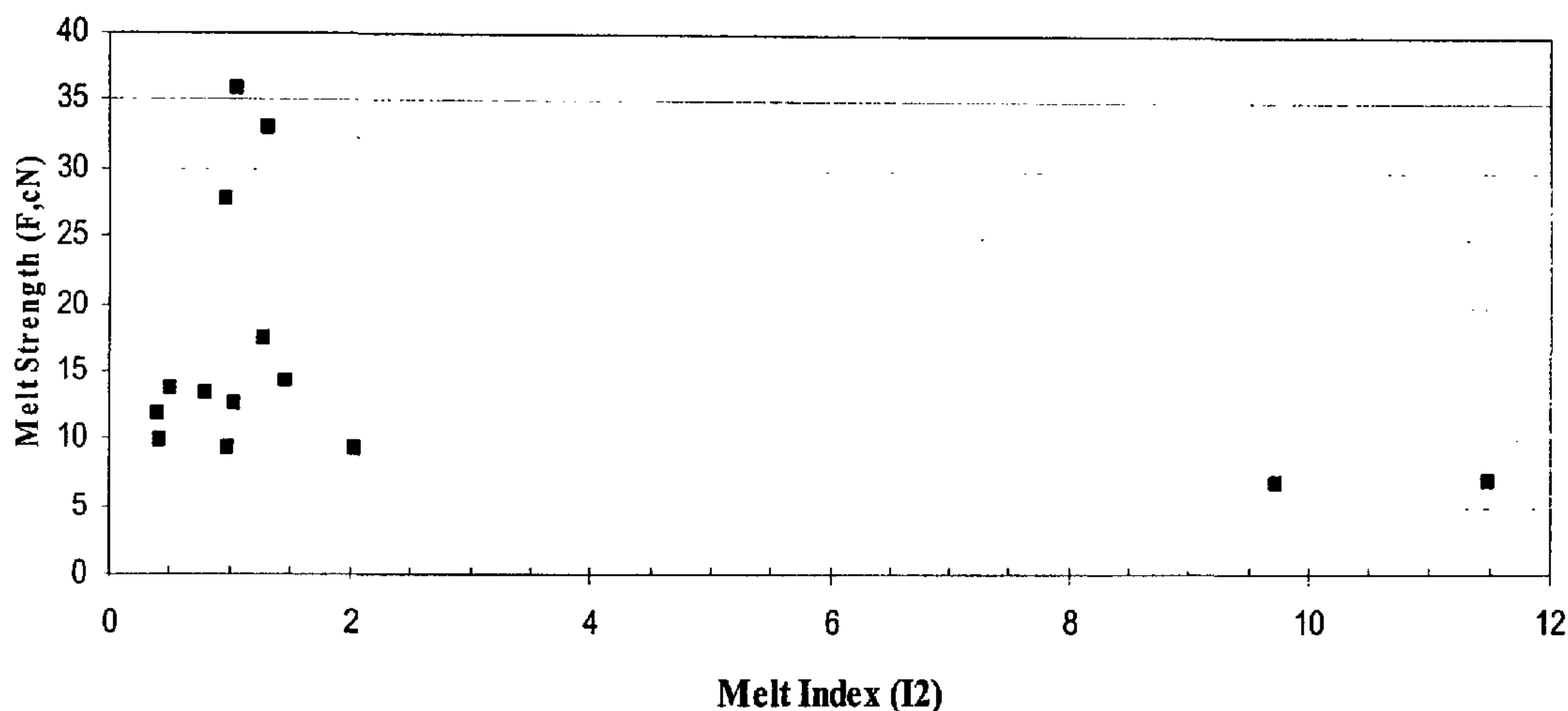
MI vs. Melt Strength Comparison
