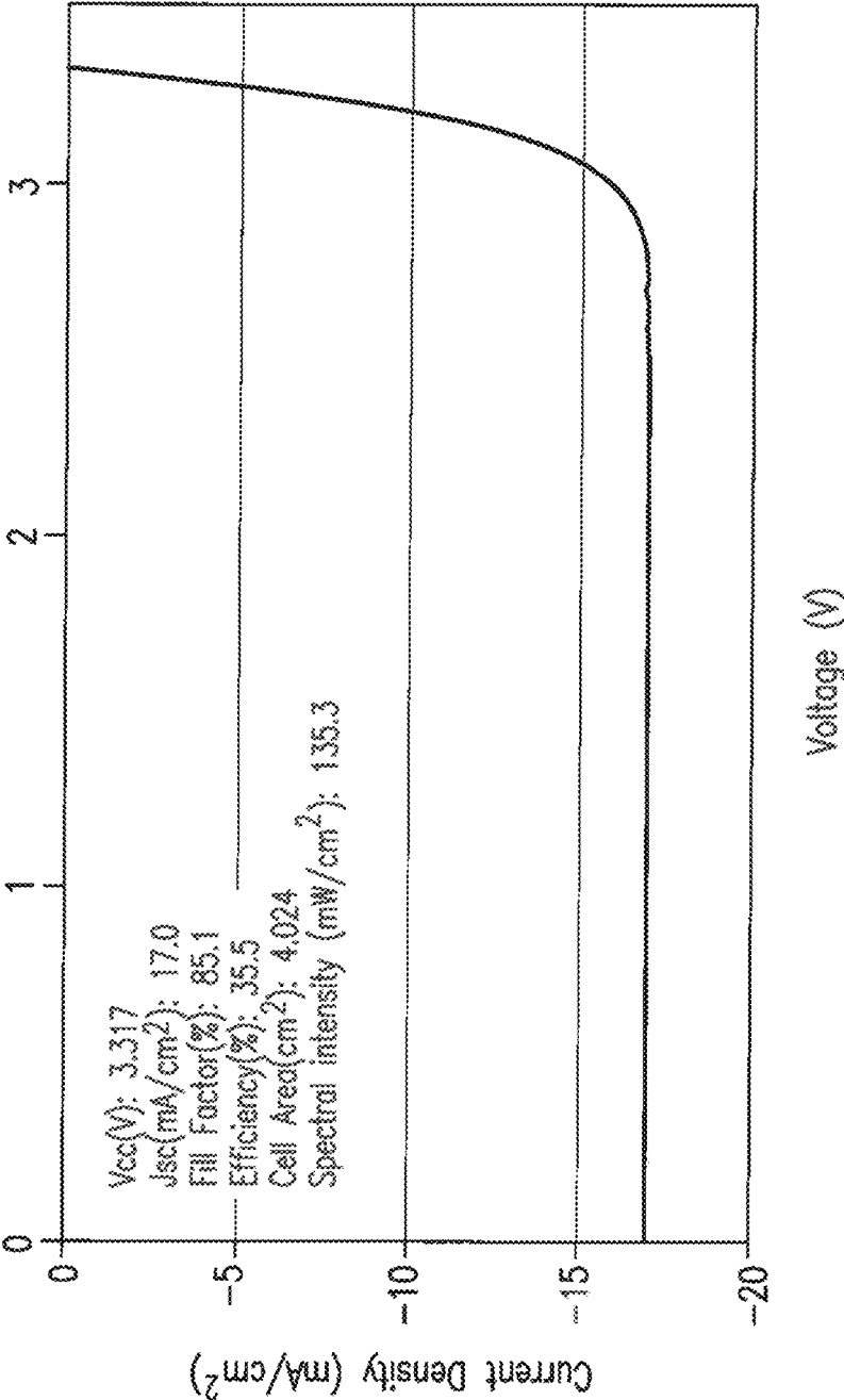
AMO JV Characteristic for 4J-IMM CELL TS572-1104
