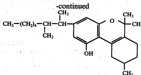
Diphenylhydantoin (DPH)
