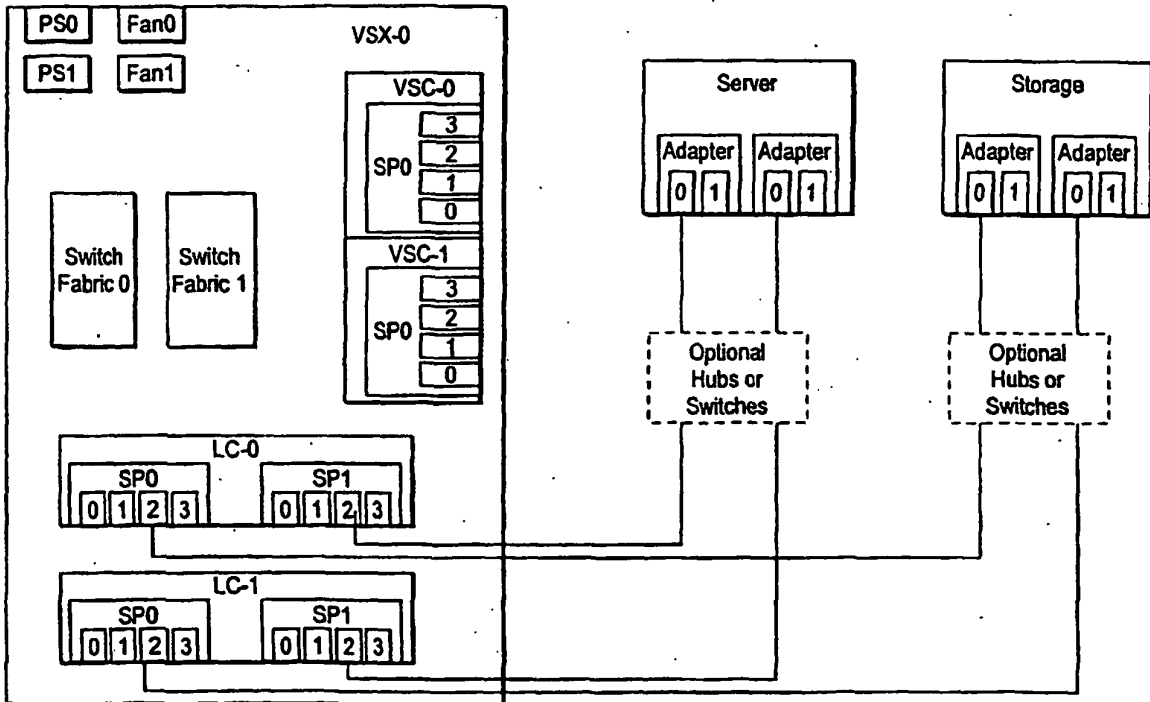
FIG. 3 Fault Tolerant Configuration
