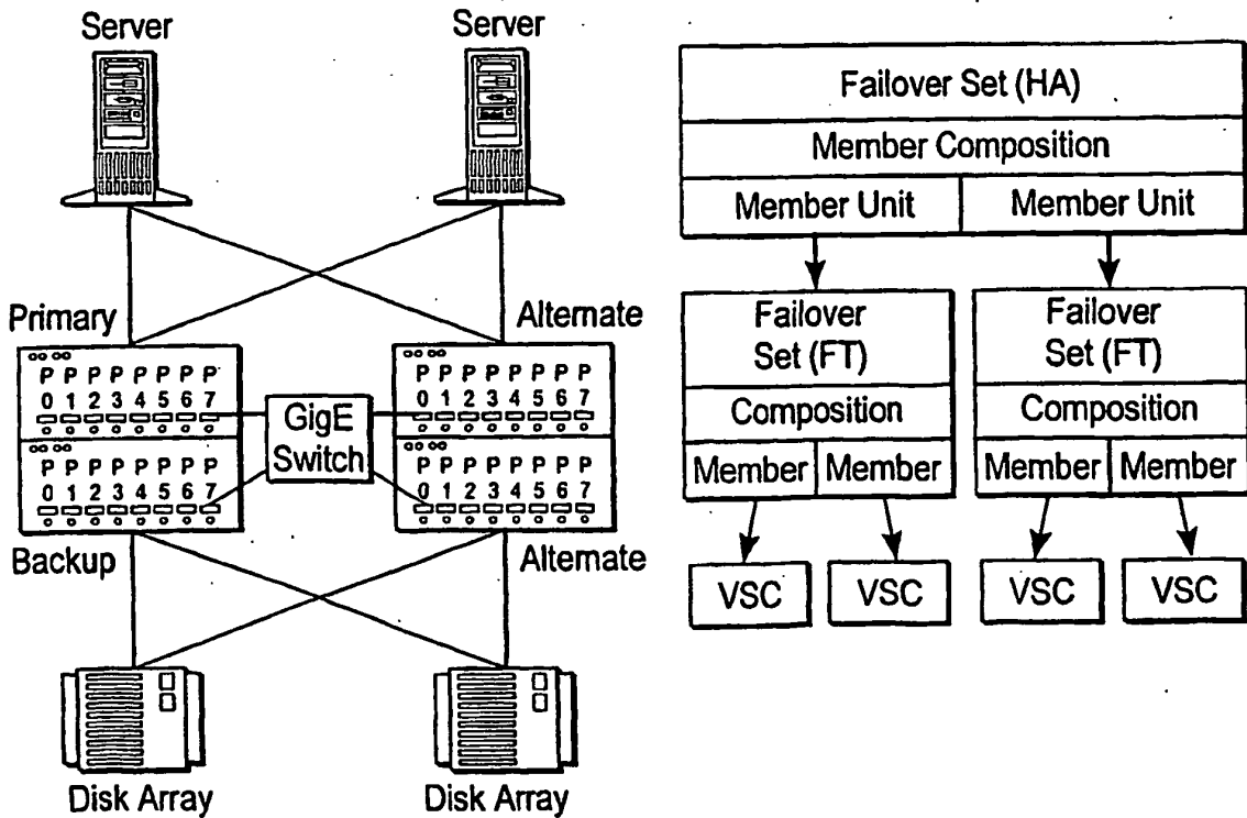
FIG. 29 Hierarchical HA Configuration
