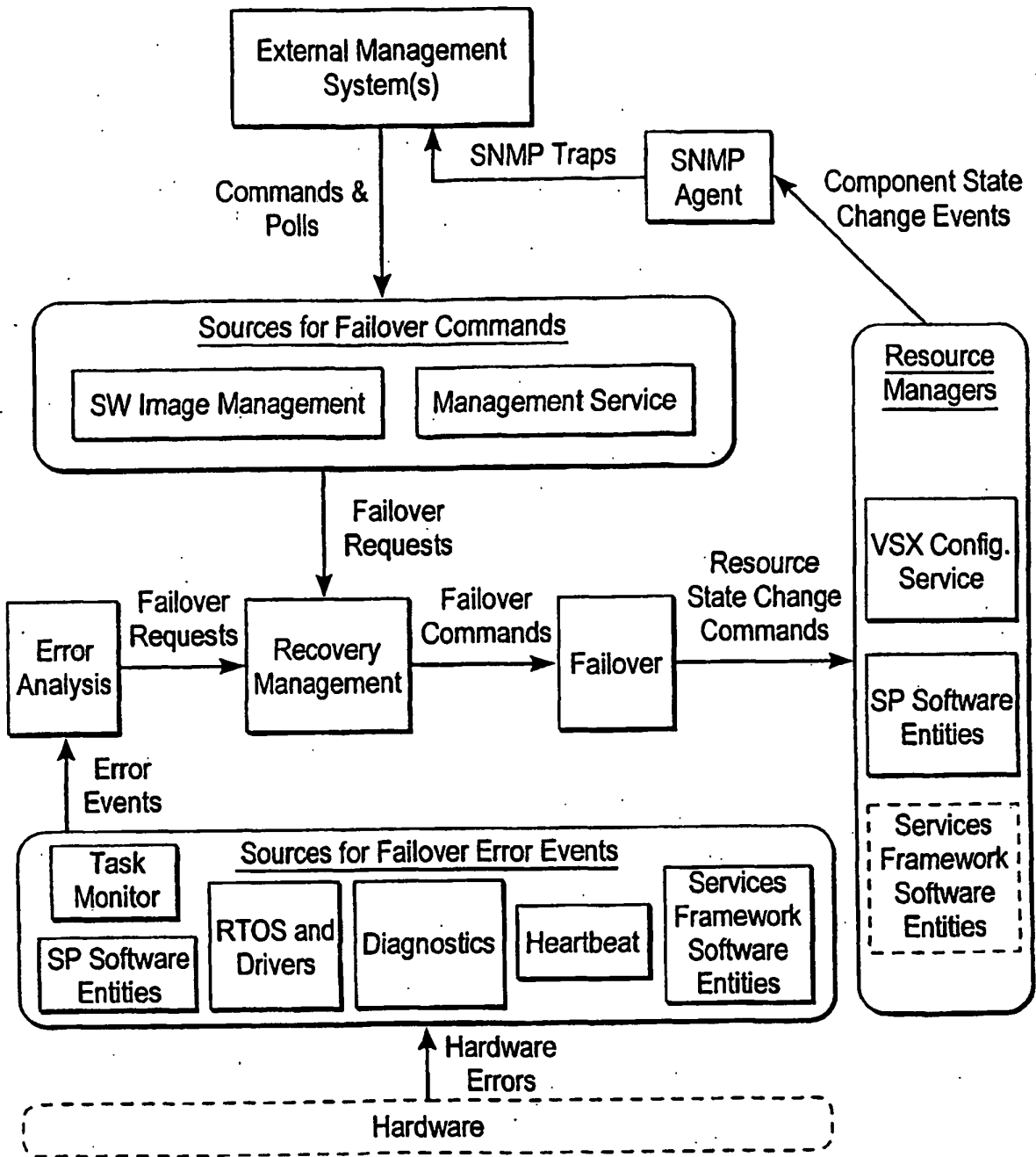
FIG. 15 Fault Detection and Analysis Architecture
