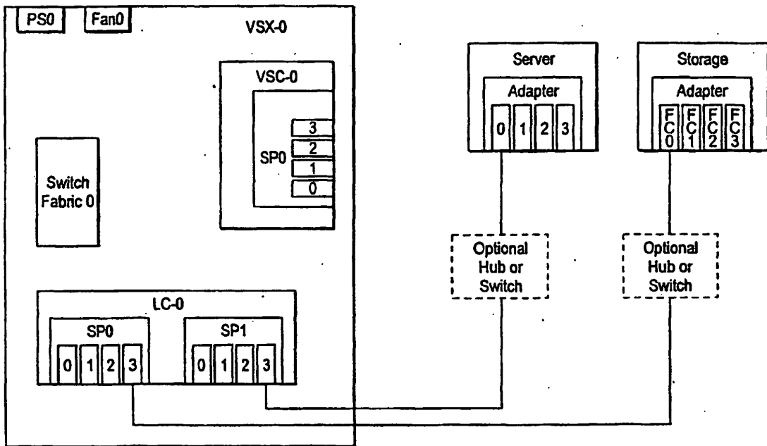
FIG. 2 Non-Fault Tolerant Configuration
