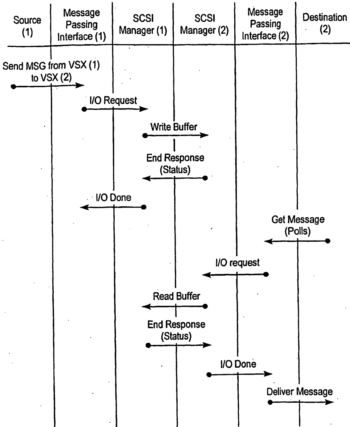
FIG. 27 VSX to VSX Communication Using Shared Disk
