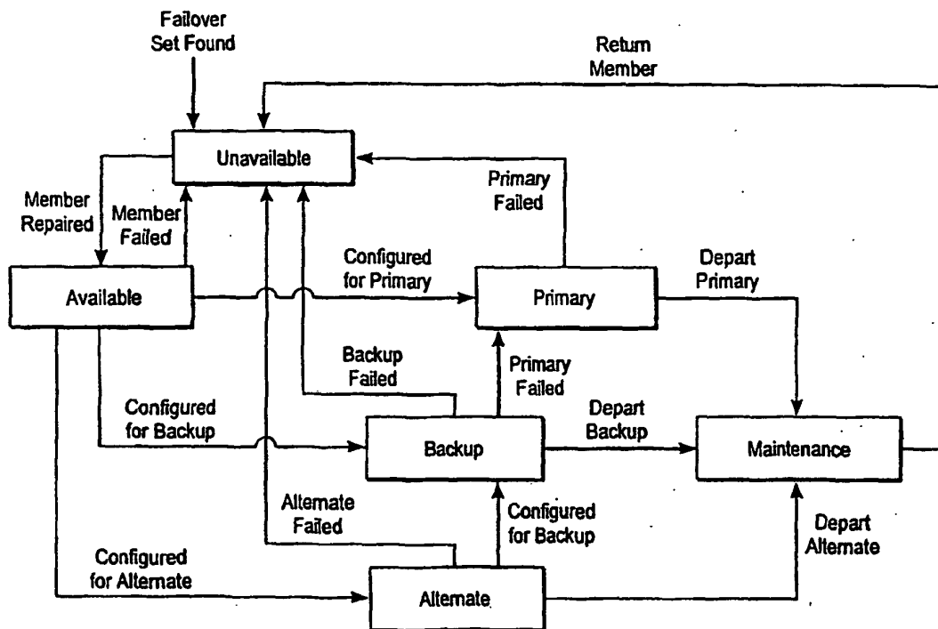
FIG. 8 Member State Diagram
