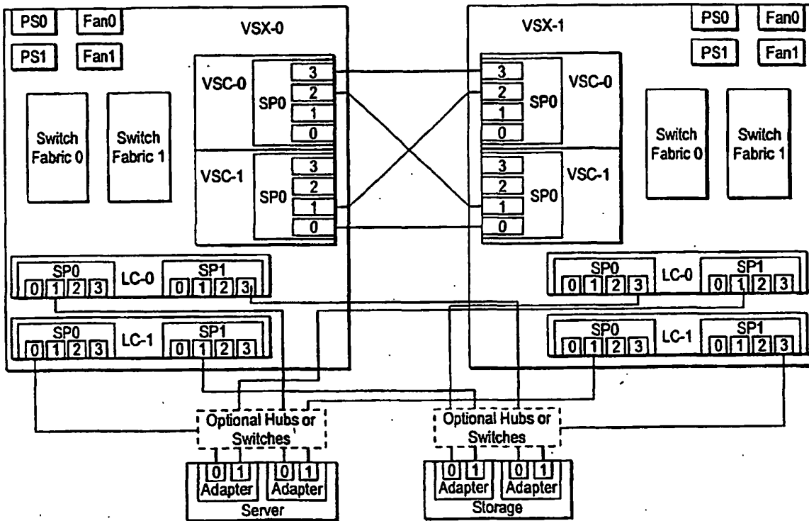
FIG. 4 High Availability Configuration
