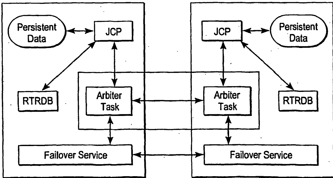
FIG. 22 An Arbiter for the Database
