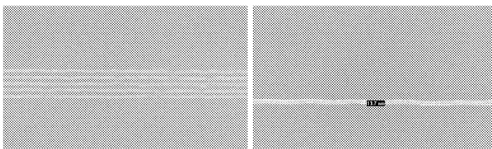
Figure 6 line dosage of 600 pC/cm
