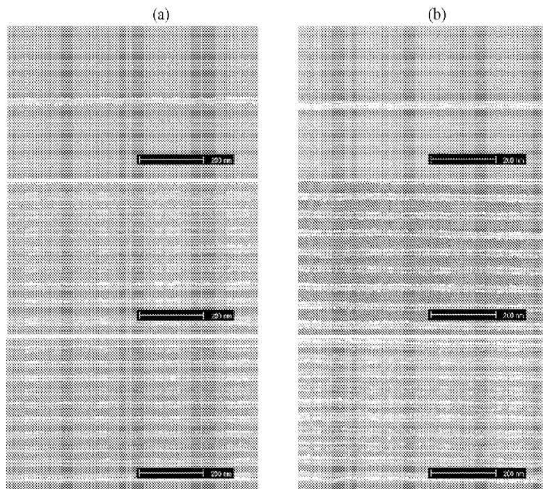
Figure 8: 15.6 nm sparse line (top), 50 nm pitch dense lines (middle) and 40 nm pitch lines
