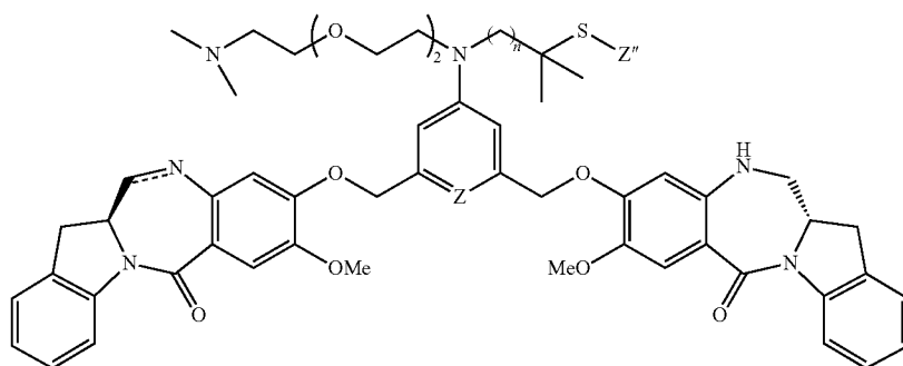
Structures of representative compounds in the present invention.
