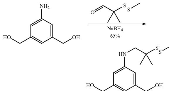
(5-(2-methyl-2-(methyl disulfanyl)propylamino)-1,3-phenylene)dimethanol
