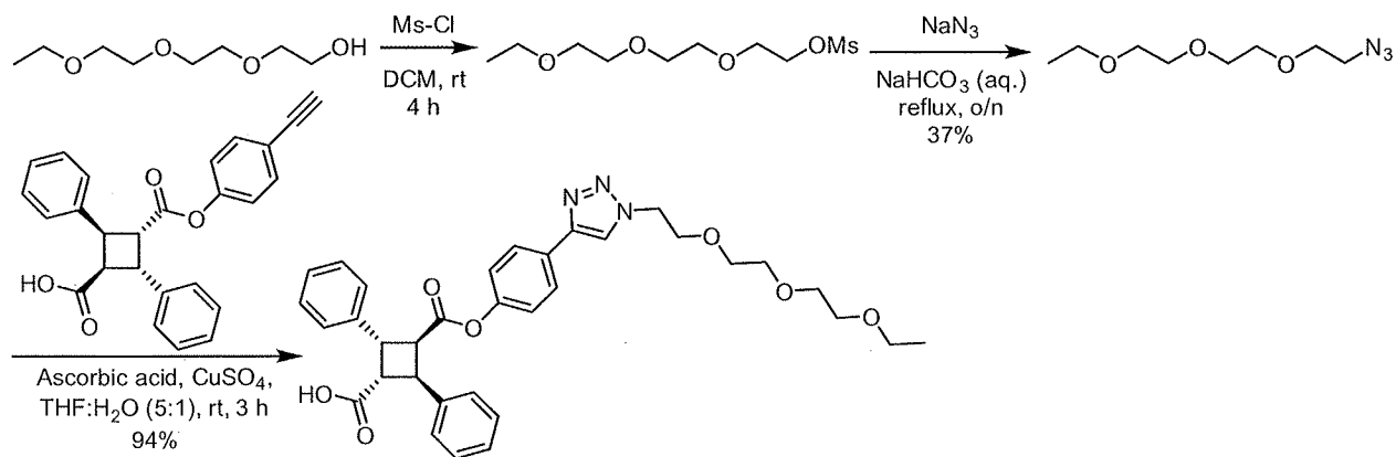
Scheme 8.
