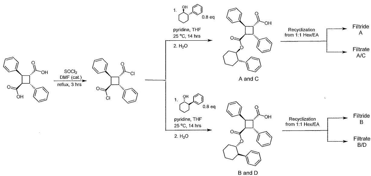
Scheme 5. Synthesis of 31 .
