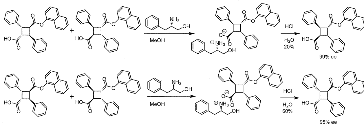
Scheme 7.
